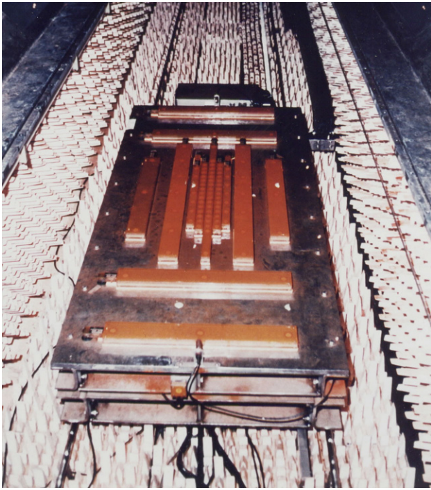
Figure 8. A photograph of the 95-element acoustic array and carriage in the LCC test section trough with the floor-mounted acoustic window removed.
