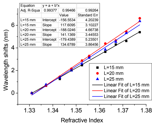
Figure 6. Measured wavelength shifts for RI sensors with L = 15, 20, and 25 mm and D = 125 \mu m in various liquids.
