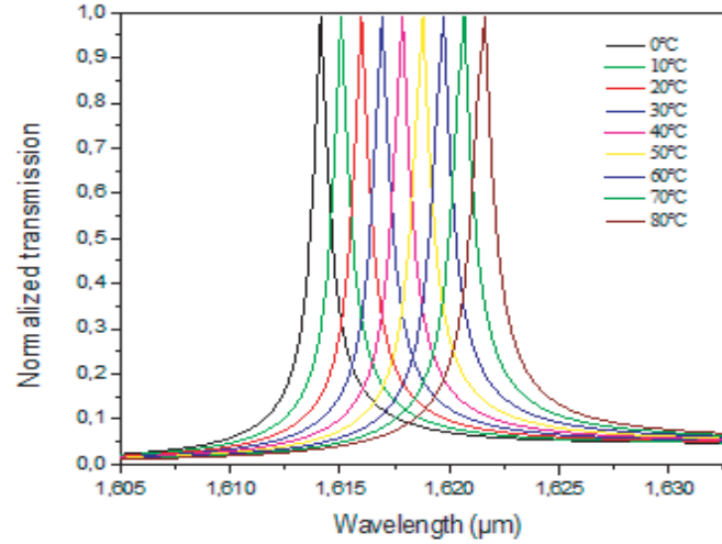
Figure 3. Transmission spectra of the proposed photonic crystal temperature sensor for different temperatures range from 0^{\circ}\text{C} to 80^{\circ}\text{C} .
