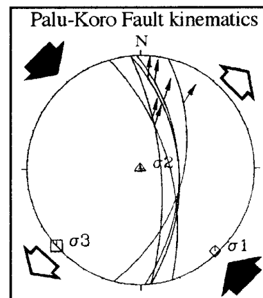
Fig. 4 Present-day fault kinematics of the northern PKF. Examples of strike-slip faulting slip data measured along the major PKF bounding the Palu basin: lower hemisphere stereoplote of fault planes and measured striations, direction arrows point in the horizontal slip azimuth direction. \sigma_1 , \sigma_2 and \sigma_3 represent the stress axes of the regionally significant stress regime obtained from the inversion of major fault striations measured around the Palu basin (Beaudouin, 1998). Large open and black arrows give the azimuths of the computed \sigma_3 and \sigma_1 , respectively.
