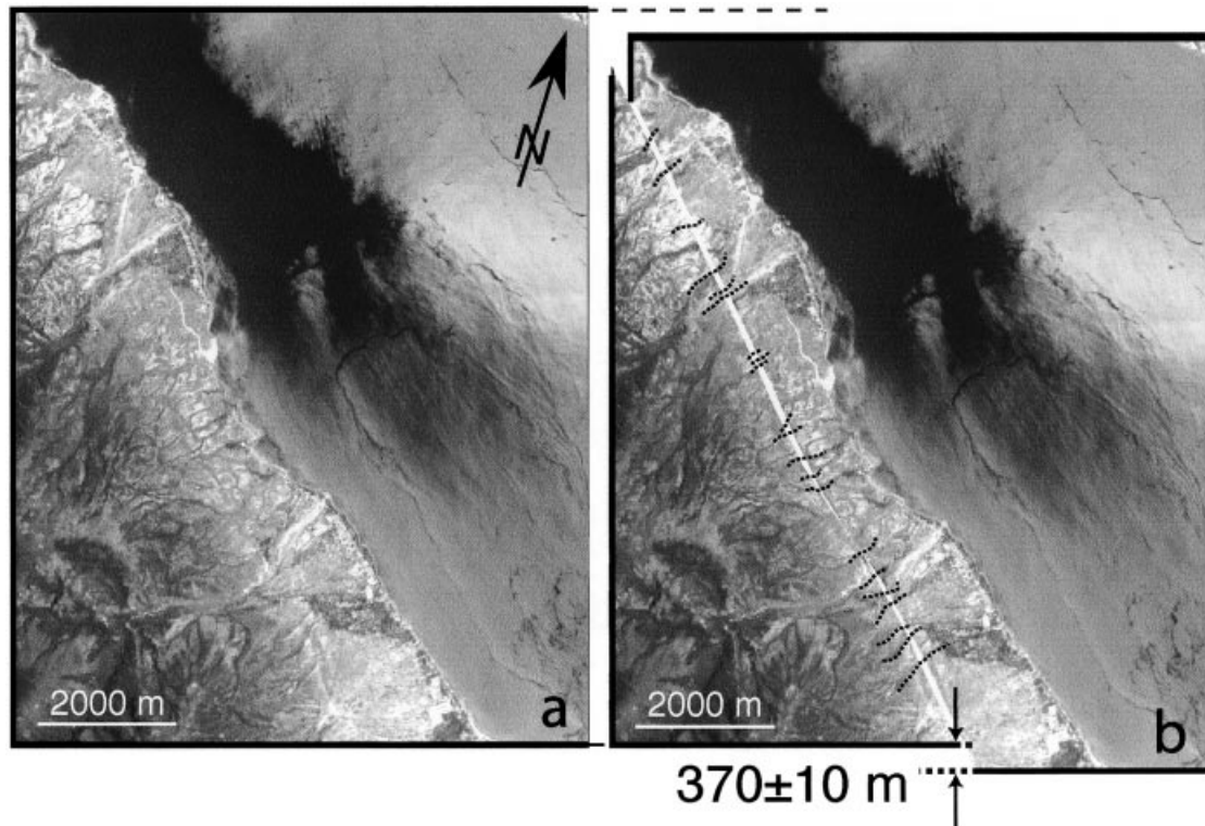
Fig. 8 Present-day (a) and restored (b) drainage along-strike PKF segments, shown on a detailed SPOT view. The restoration involves an offset of 370 \pm 10 m. Location: see Fig. 6.
