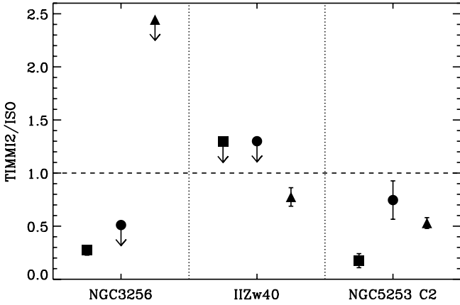
Fig. 7. Comparison between the line fluxes measured by TIMM12 and ISO. Symbols correspond to [Ne II] 12.8 \mu m (square), [Ar III] 9.0 \mu m (circle) and [S IV] 10.5 \mu m (triangle). The lines are ordered by increasing ionisation potential: 21.6, 27.6 and 34.8 eV respectively. In the case of NGC 3256, we have added the contributions of the N and S nuclei to the TIMM12 flux since the ISO aperture includes both sources. The dashed line represents the one-to-one relation.
