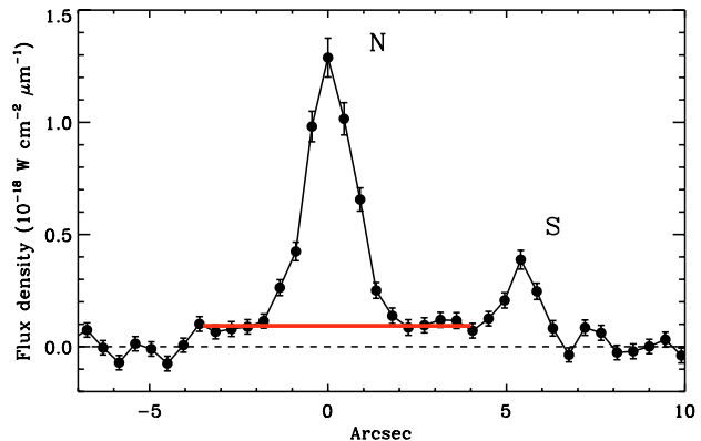
Fig. 1. Spatial variation of the [Ne II] line peak across the slit from north (left) to south (right). Error bars indicate 1\sigma errors. A plateau which extends over \sim 8'' is indicated by a solid line in light colour. At the distance of NGC 3256, 1'' corresponds to \sim 179\ \text{pc} . The peak positions of the northern and southern nuclei are identified by the labels N and S respectively.
