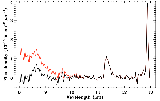
Fig. 3. Continuum subtracted spectrum of NGC 3256 N. The result of using the two extreme possibilities for the continuum plotted in Fig. 2 is shown by the dark and light lines. Note that the difference in both continua is the removal or not of the underlying PAH plateau and wing of the 7.7 \mu\text{m} complex (see Fig. 4).
