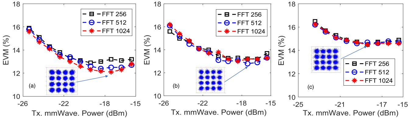
Fig. 4. Performance of OFDM signal for different FFT sizes and fiber transmission lengths: (a) 10-km SMF; (b) 20-km SMF; (c) 30-km SMF.
