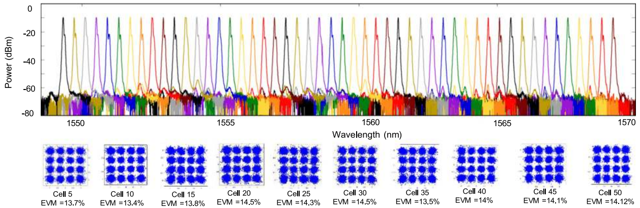
Fig. 8. Spectra of switched optical SSB signals and examples of signal performance at different cells.
