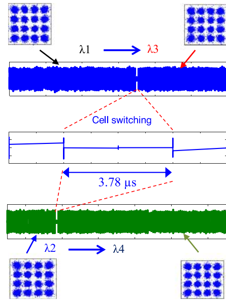
Fig. 7. Cell switching by the wavelength-tunable lasers.
