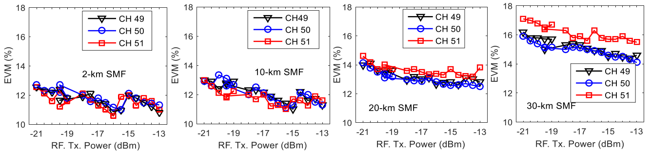
Fig. 10. Uplink signal performance for different RF transmit powers and different fiber lengths.
