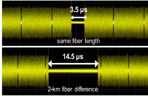
Fig. 12. The interrupted time during radio cell switching.
