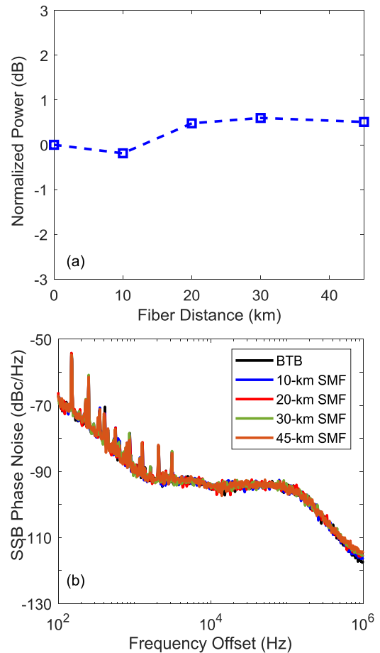
Fig. 3. (a) LO normalized power; and (b) SSB phase noise characteristics.
