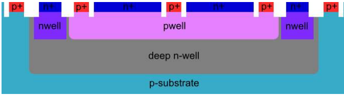
Fig. 8. A potential APD structure as reported in [23].
