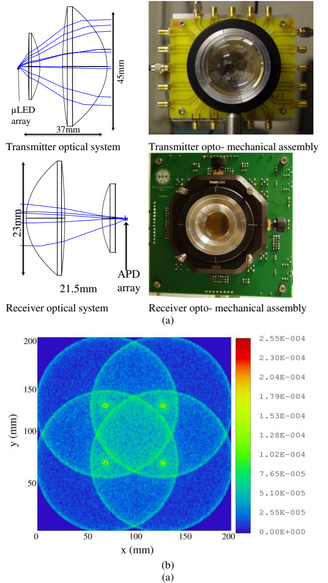
Fig. 5. a) Schematic of optical system and snapshot of the opto-mechanical assemblies b) simulated optical irradiance ( \text{W}/\text{cm}^2 ) in a 200 \times 200 \text{ mm}^2 receiver plane at 1 m distance from the transmitter.
