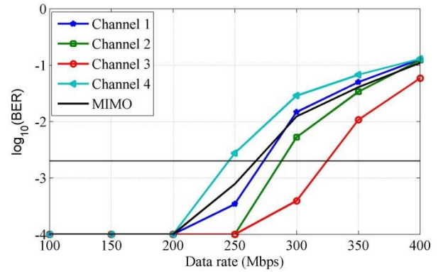
Fig. 10: Data rates against the BER for individual channel and aggregate MIMO system. Note that MIMO data rate is divided by 4 for the clarity of the figure.
