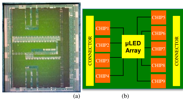
Fig. 6. \mu LED driver a) fabricated die and b) transmitter PCB block diagram.
