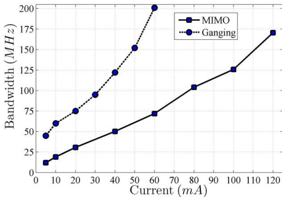
Fig. 9. Measured electrical-to-electrical bandwidths against the bias current of ganging and MIMO devices.
