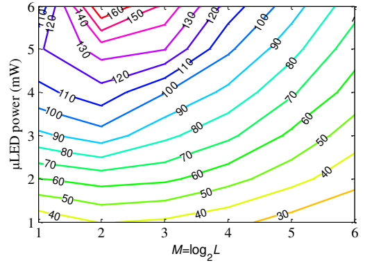
Fig. 4. A contour plot of the maximum achievable data rates (Mbps) using L -PAM for different \mu LED powers.
