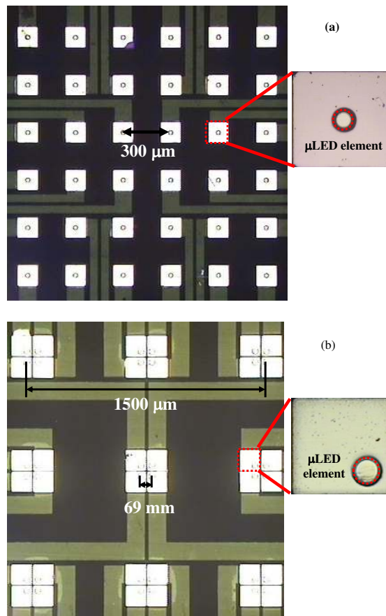
Fig. 7. a) Images of a) \mu LED array of the ganging device and b) \mu LED array of the MIMO device. High-magnification images for typical \mu LED elements are also shown.
