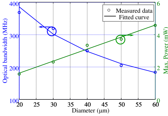
Fig. 2. The relationship among the optical bandwidth, optical power and \mu LED diameter. The measured data and fitted curves are also shown.
