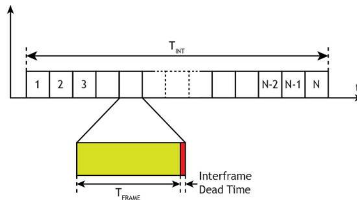
Fig. 1. Typical acquisition scheme for the adopted SPAD array: given the absence of readout noise and short inter-frame dead time, longer integration time can be obtained by accumulating several shorter frames. The dynamic range is correspondingly increased.
