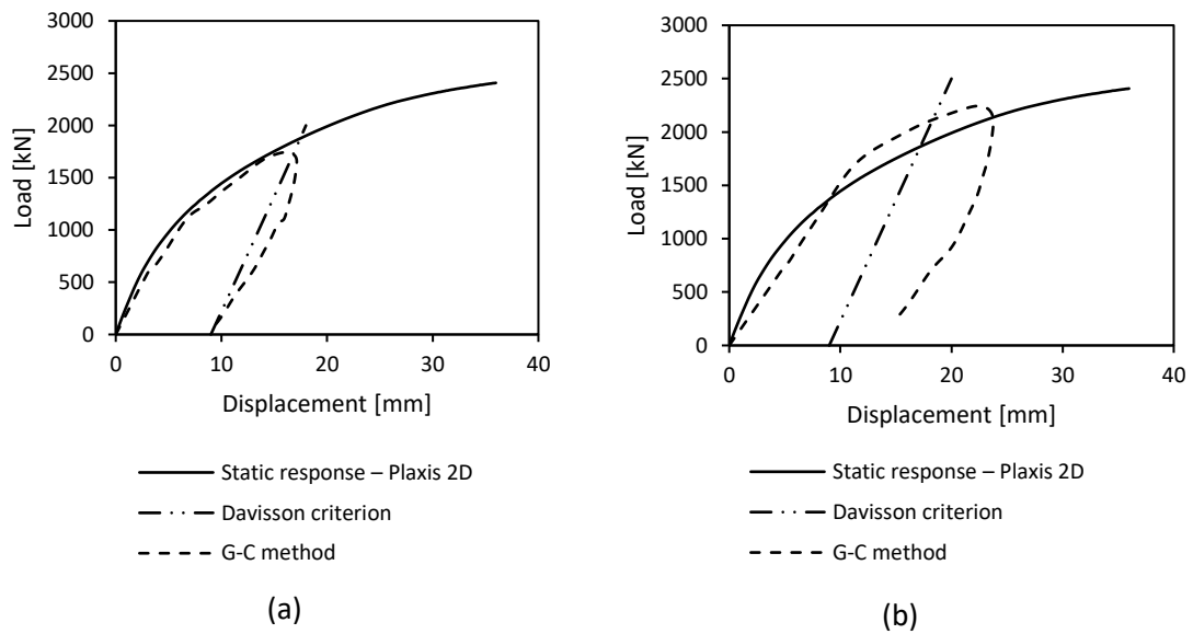
Figure 4- 36: Responses of piles at different values of Ks for Case 2: (a) 3E08 N/m, (b) 3E09 N/m.
