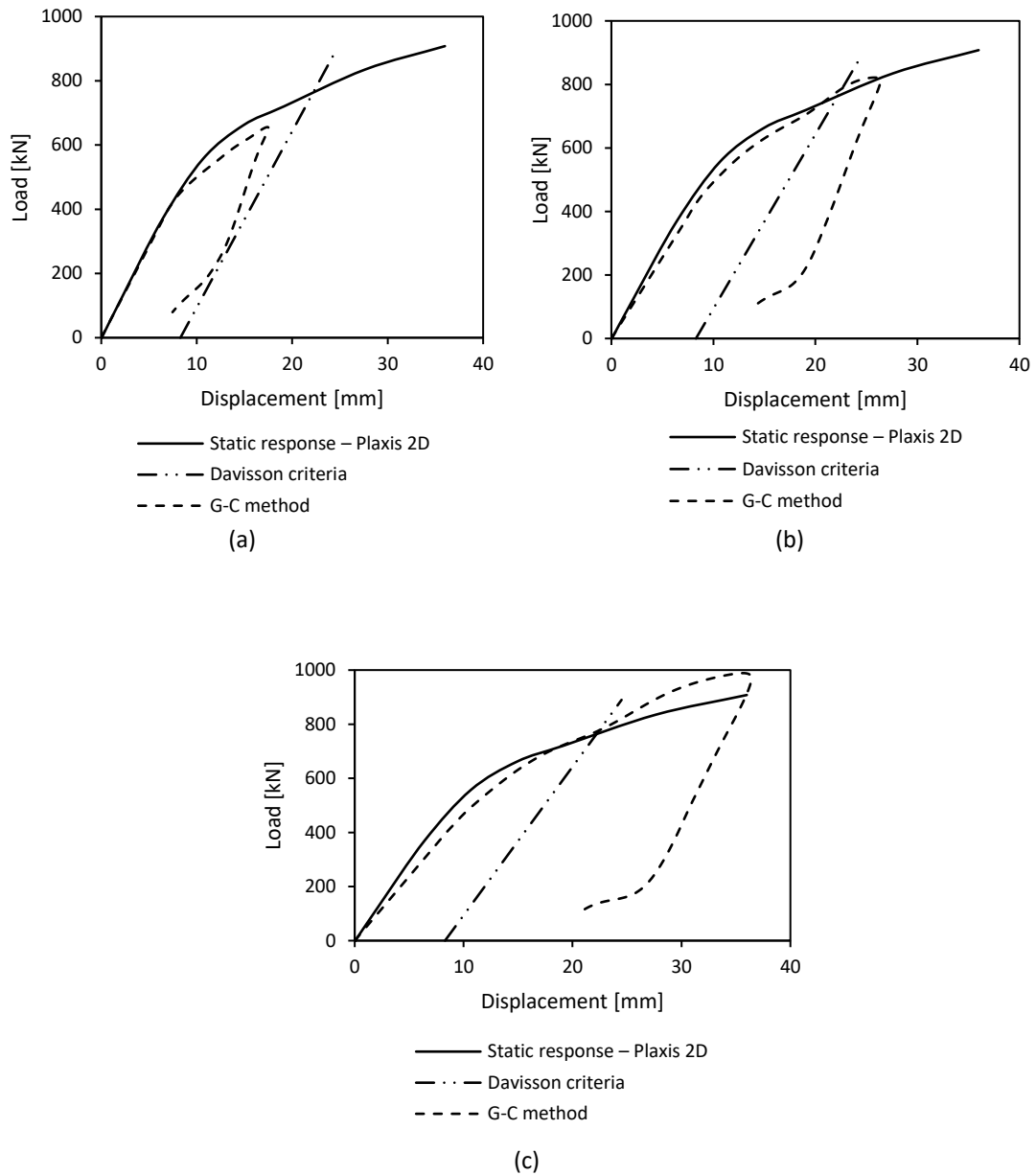
Figure 4- 27: Load-displacement curves obtained from dynamic and static simulations for different hammer drop heights for piles installed in sand: (a) 0.9 m; (b) 1.5 m; (c) 2 m.
