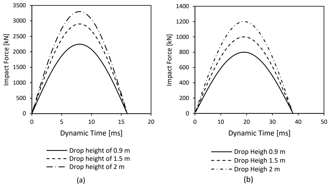
Figure 4- 26: Shape of force pulses generated at different heights: (a) for single-helix pile installed in sand, and (b) for the double-helix pile installed in clay.
