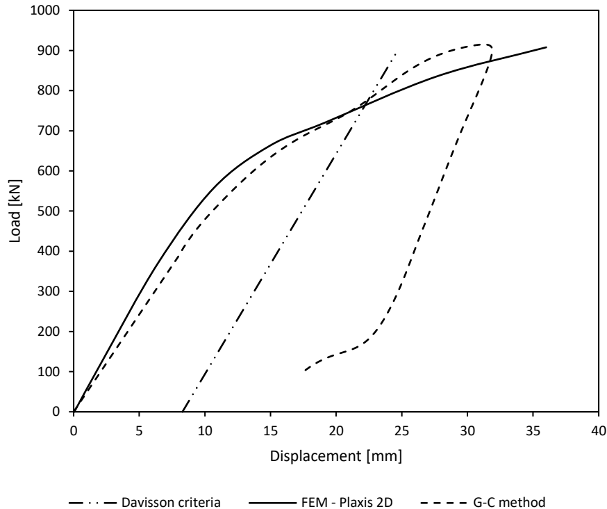
Figure 4- 18: Load-displacement curves from numerical model and G-C method – Case 1.
