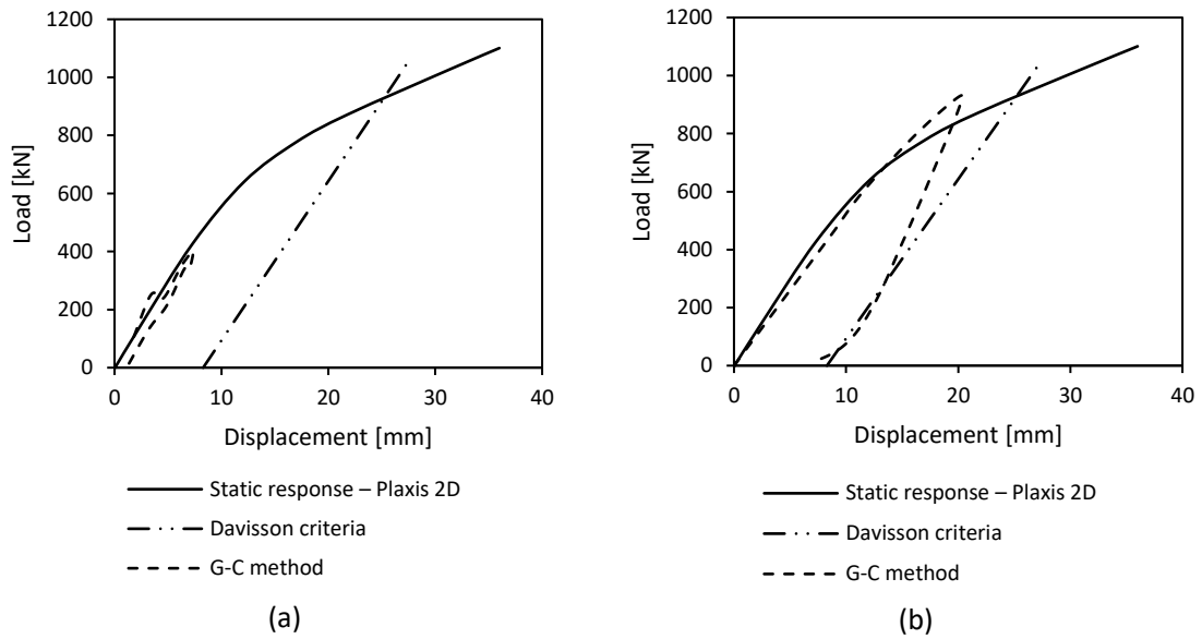
Figure 4- 35: Responses of the helical pile to different values of Ks for Case 1: (a) 8E06 N/m, (b) 8E07 N/m.
