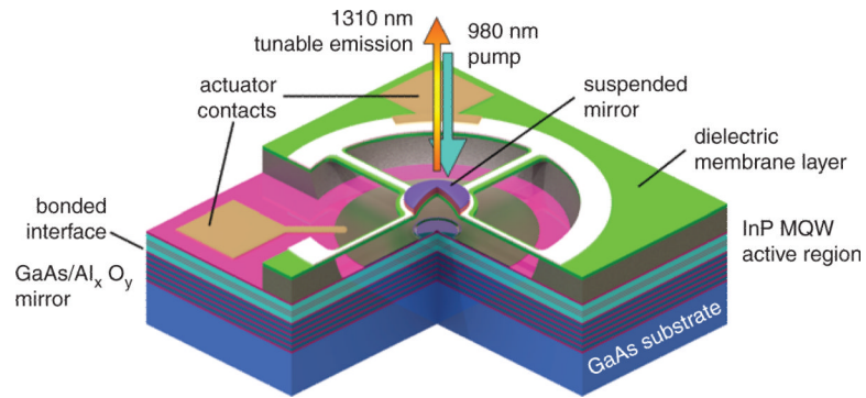
Fig. 1. Solid model of device structure employed in this work, combining wide-bandwidth long-wavelength active region with optimised tunable microcavity
