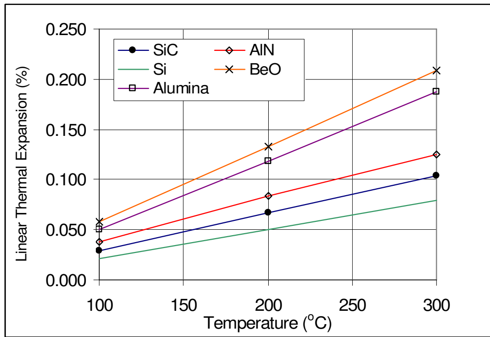
Fig. 8. Thermal expansion of common ceramics and device materials vs. temperature [38].
