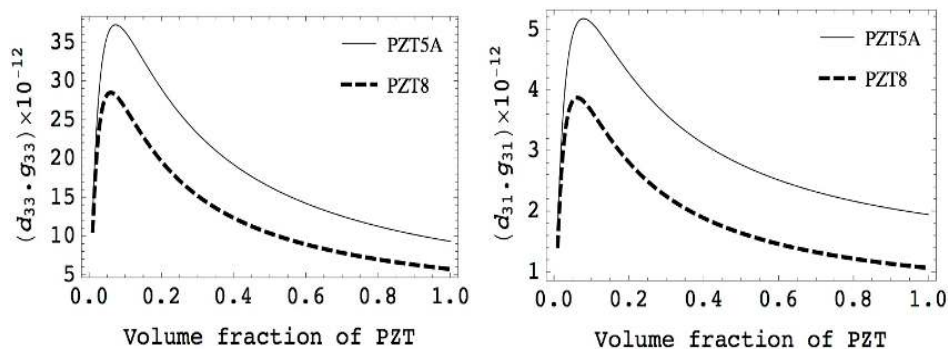
Figure 5. Computed figure-of-merits ( d_{33} \cdot g_{33} and d_{31} \cdot g_{31} ) for transducers and sensors as a function of piezoelectric volume fraction for PZT5A and PZT8.
