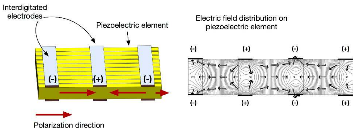
Figure 3. Schematic of fiber composite actuator (Left); Electric field distribution on piezoelectric element, where arrow indicates the direction of electric field (Right).
