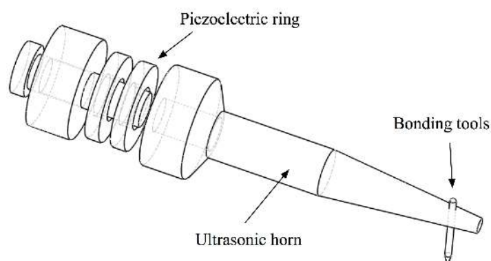
Figure 10. Schematic representation of the ultrasonic wire-bonding device.
