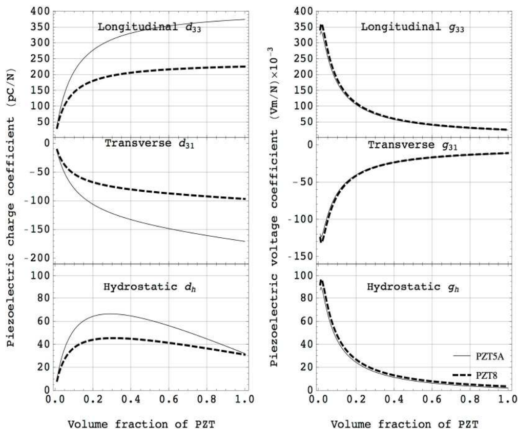
Figure 4. Computed piezoelectric charge, voltage and hydrostatic coefficients as a function of volume fraction for PZT5A (solid line) and PZT8 (dashed line).
