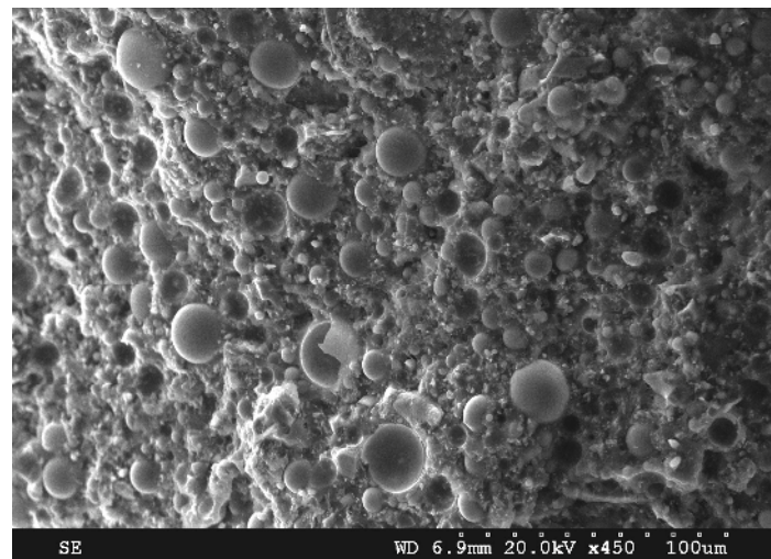
Figure 11. SEM cross-sections of a glass sphere modified epoxy.
