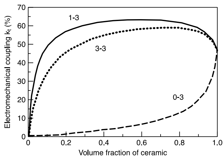
Figure 1. Electromechanical coupling factors of 1-3, 3-3 and 0-3 piezocomposites as a function of volume fraction of piezoelectric ceramic (Reprinted with permission from [45]. © [1998] IEEE.).
