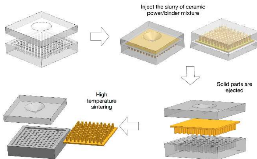
Figure 7. 1-3 piezocomposite fabrication using the injection molding technique.
