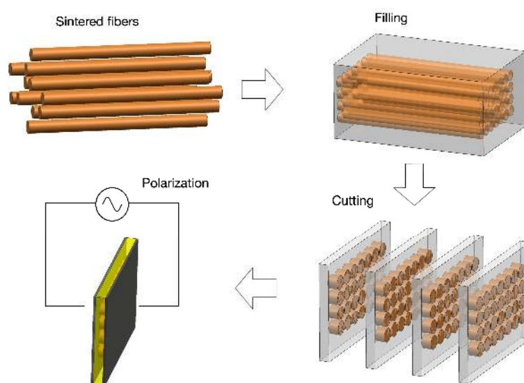
Figure 6. Process chart of 1-3 fiber composite fabrication process.
