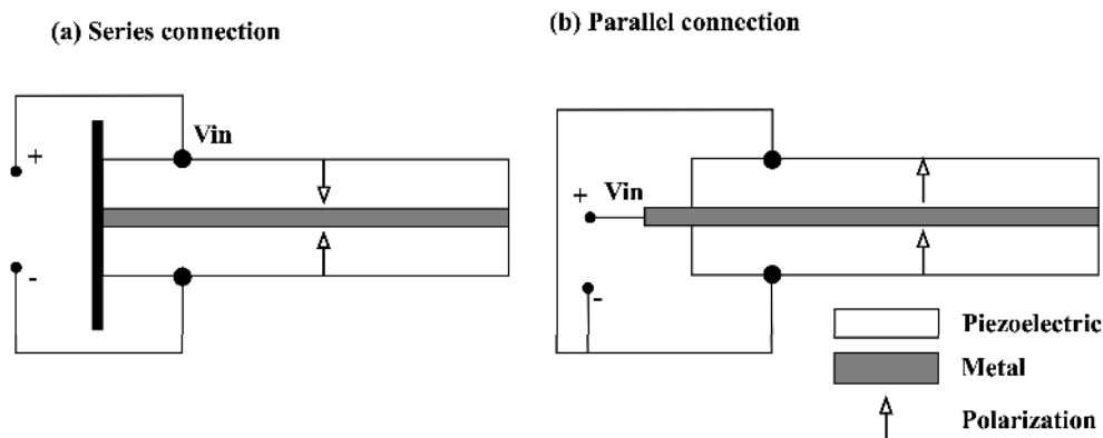
Figure 12. Schematic diagram of bimorph composites energy harvester with (a) series and (b) parallel connections.
