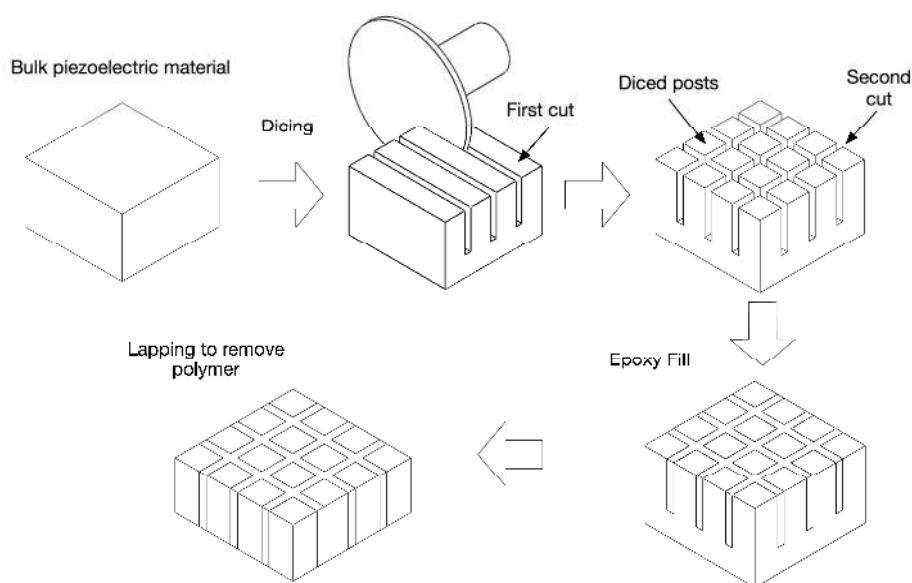
Figure 8. 1-3 composite fabrication using the dice-and-fill technique.
