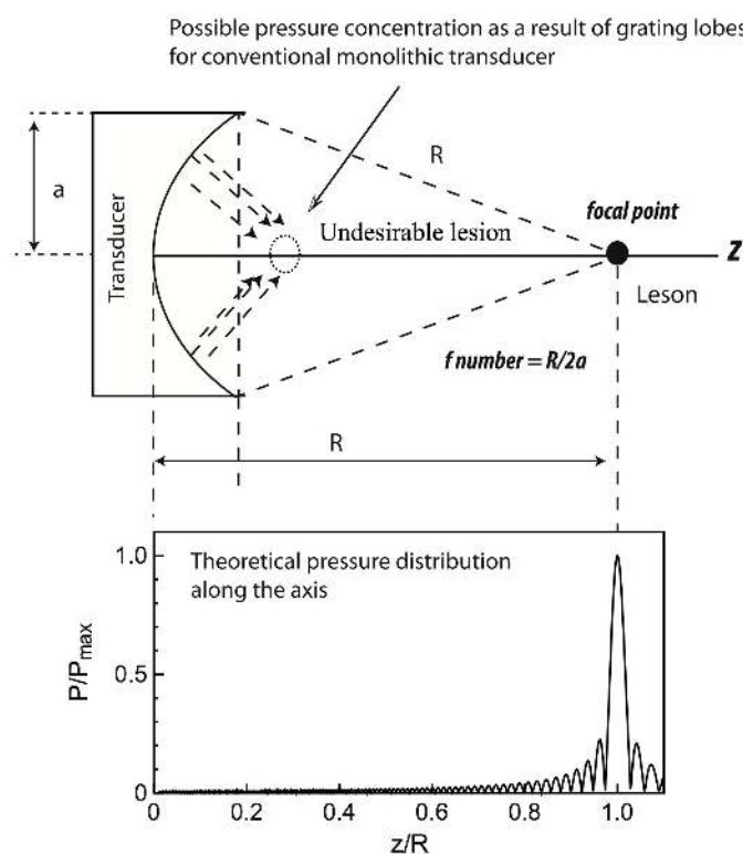
Figure 9. Theoretical on-axis normalized axial pressure profile from spherically focused ultrasound transducers whose radius of curvature is R .
