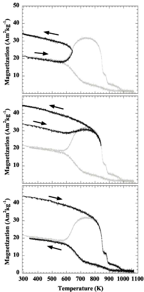
FIG. 7. Heating-cooling M(T) cycles up to selected temperatures in order to show the different zones for irreversibility and reversibility of the magnetization of the fcc- \text{Fe}_{16}\text{Cu}_{84} . The curves are compared with the M(T) curve of the segregated sample shown in Fig. 5. The arrows indicate the heating and cooling measurements.
