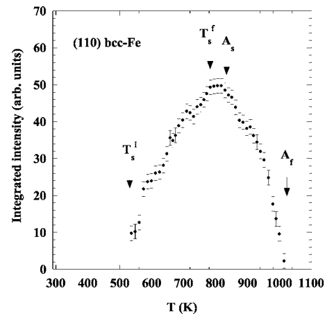
FIG. 3. Temperature dependence of the integrated intensity of the (110) reflection of bcc-Fe-rich phase segregated from the fcc- \text{Fe}_{16}\text{Cu}_{84} solid solution during the first heating process.
