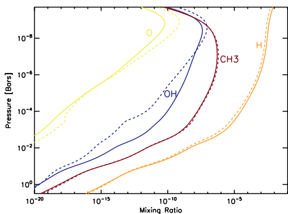
Figure 4. Important radical species involved in pathways governing the abundances of CH 4 , H 2 O, CO, and CO 2 . Solid is for the dayside temperature profile, dashed is for the nightside temperature profile. The abundances of radicals increase with decreasing pressure due to the availability of dissociating photons higher in the atmosphere.
