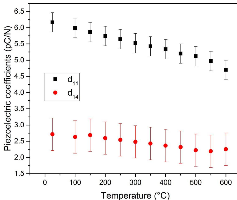
Fig. 4. Temperature dependence of the piezoelectric strain constants d_{11} and d_{14} . The error bars are the standard deviation (close to 0.3 pC/N for d_{11} and 0.5 pC/N for d_{14} ).
