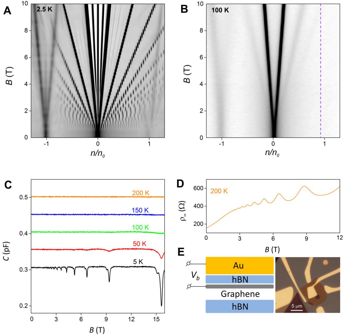
Figure S5 | Differential capacitance for graphene superlattices. a , Low- T Landau fan diagram C(n, B) for a capacitor with a \approx 13.5 nm. Grey linear scale: black 0.266 pF; white 0.293 pF. b , Same as in (a) but at 100 K. Scale: black 0.328 pF; white 0.357 pF. c , Examples of C(B) for the fixed n \approx 2.3 \times 10^{12} \text{ cm}^{-2} ( n/n_0 \approx 0.9 ) which corresponds to the purple dashed line in (b). The curves are shifted vertically for clarity. d , \rho_{xx}(B) for a Hall bar device with a \approx 13.9 nm and measured at the same n and T as the orange curve in (c). e , Schematic and optical image of one of our capacitance devices. For details, see ref. 20.
