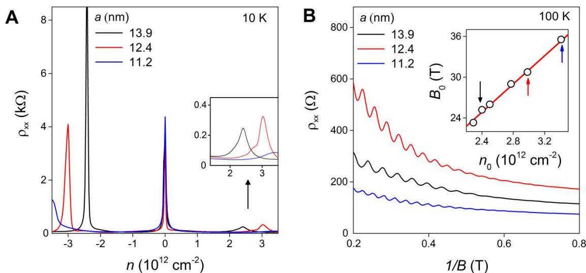
Figure S3| Frequency of Brown-Zak oscillations for different graphene superlattices. a, Examples of characterization of our superlattice devices. The second-generation NPs are found at \pm n_0 which can be translated into the values of a and S for the superlattices 17-25 . Inset: Behavior near the electron NPs is magnified. b, BZ oscillations for the three devices in (a) at approximately the same normalized density n/n_0 \approx 0.75 . Inset: Frequency B_0 of the BZ oscillations for all our superlattice devices as a function of the position of their NPs (symbols). This includes the devices in (a,b) as indicated by the color-coded arrows. Red line: Expected dependence B_0 = \phi_0 n_0/4 . B_0 corresponds to the last maximum in \sigma_{xx} that should appear at one \phi_0 per superlattice unit cell.
