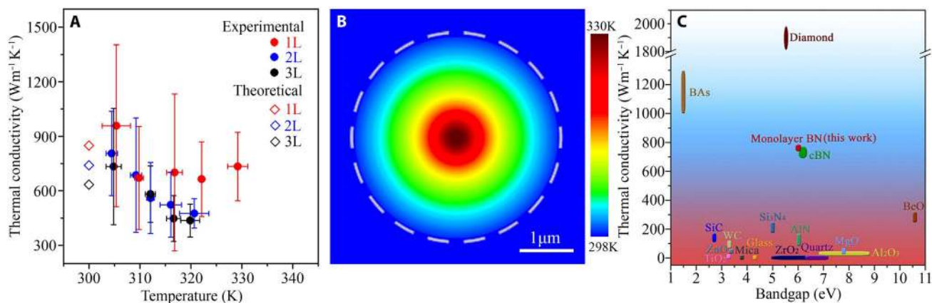
Fig. 4. Thermal conductivity of 1-3L BN. (A) Experimental \kappa of the suspended 1-3L BN as a function of temperature (filled circles) and the corresponding theoretical values at 300 K (open rhombus). (B) Temperature distribution of a suspended 1L BN over 3.8- \mu m microwells under laser heating up to 330 K with the heat sink kept at 298 K, and the dashed circle represents the edge of the suspended BN. (C) Comparison of the thermal conductivity of some common semiconductors and insulators.
