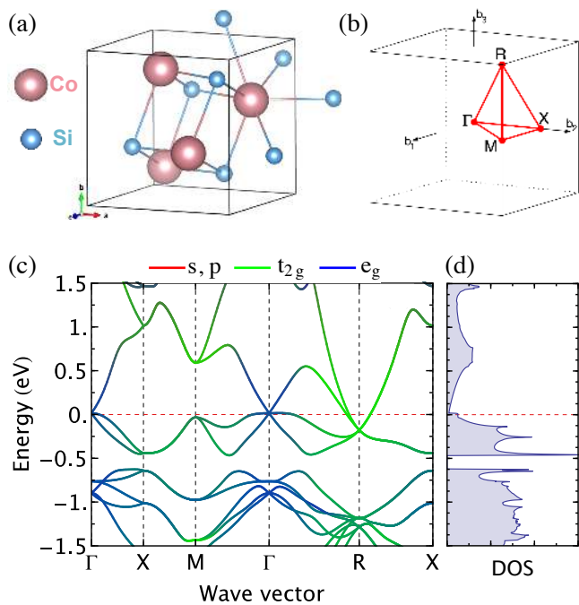
FIG. 1. (a) Crystal structure, (b) Brillouin zone with high symmetry points, (c) Electronic band structure and (d) Density of states (DOS) of B20 -type \text{CoSi} . The Co and Si atoms are colored in red and blue respectively. The band structure is color coded according to different orbitals shown in the legend, namely, s , p , e_g and t_{2g} states.
