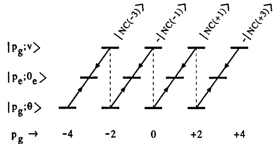
FIG. 2. The transition scheme for Q=4 . The nonorthogonal states that comprise the superposition are denoted by v and \theta , and the various ground-state momentum values are indicated. The index n corresponds to P , the odd-integer, excited-state momenta.
