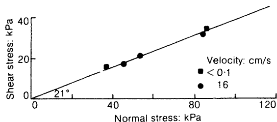
Fig. 6. Strength envelopes of the polystyrene beads
