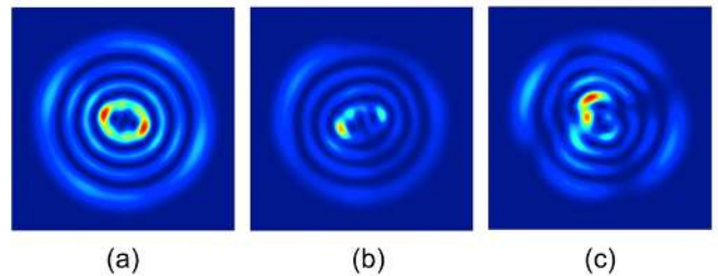
FIG. 4. LG_{3,3} simulated transverse intensity distributions at (a) cavity transmission, (b) reflection and (c) at the interferometer output when the cavity is at resonance and the Michelson is set on the dark fringe. Window side is 6 mm. Same colorscale for the three figures.
