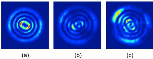
FIG. 3. LG_{3,3} measured transverse intensity distributions at (a) cavity transmission, (b) reflection and (c) at the interferometer output when the cavity is at resonance and the Michelson is set on the dark fringe. Window side is 6 mm. Same colorscale for the three figures.
