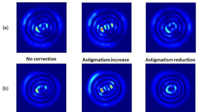
FIG. 9. LG_{3,3} Transverse intensity distributions measured (a) and simulated (b) at cavity reflection. Left column: reference condition (presented in section III). Central column: astigmatism enhancement. Right column: astigmatism reduction. The colour scale is the same for the three configuration.
