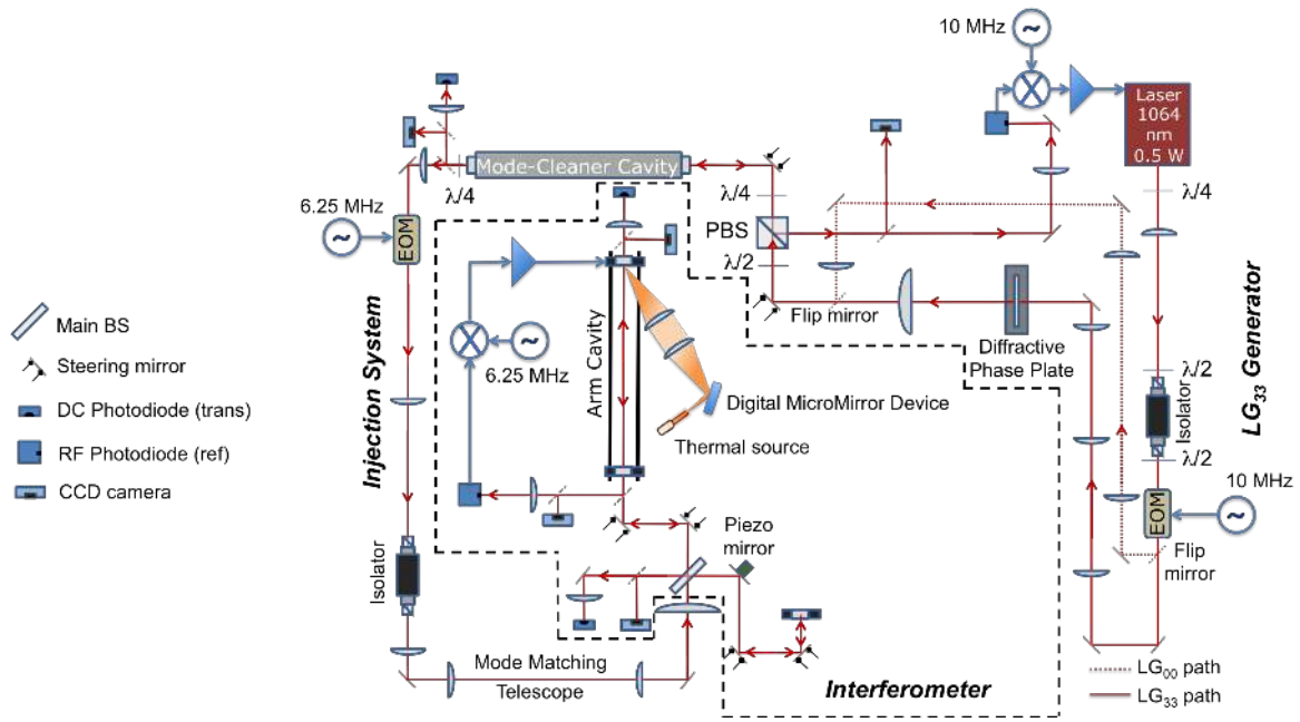
FIG. 1. Scheme of the experimental set-up.
