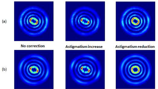
FIG. 8. LG_{3,3} Transverse intensity distributions measured (a) and simulated (b) at cavity transmission. Left column: reference condition (presented in section III). Central column: astigmatism enhancement. Right column: astigmatism reduction. The color scale is the same for the three configuration.
