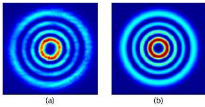
FIG. 2. Normalized intensity distribution recorded at the mode cleaner output (a) and theoretical LG_{3,3} distribution at the same distance from waist (b).
