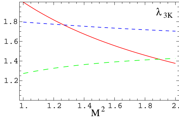
Figure 7: \lambda_{3K} as a function of the Borel parameter, calculated from the non-diagonal sum rule (C.16) (red, solid line), the pure-parity diagonal sum rule (C.14) (green, long dashes) and the mixed-parity diagonal sum rule (C.15) (blue, short dashes); s_0 = 1.1 \text{ GeV}^2 ; \lambda_{3\pi} = 0 by virtue of G-parity.
