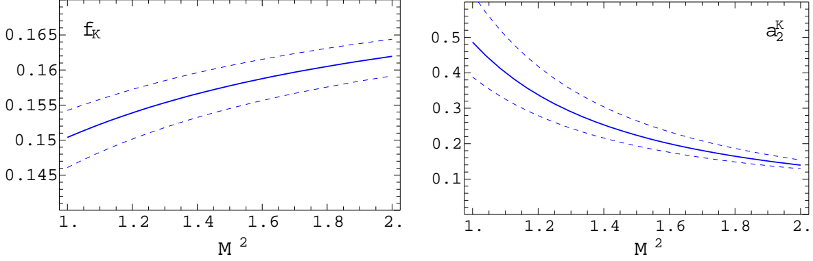
Figure 4: Left panel: f_K as function of the Borel parameter M^2 for s_0 = 1.1 \text{ GeV}^2 . Solid line: central values of input parameters, dashed lines: variation of f_K within the allowed range of input parameters. Figure taken from Ref. [10]. Right panel: same for a_2^K at the scale \mu = 1 \text{ GeV} . The results for a_2^K are new.
