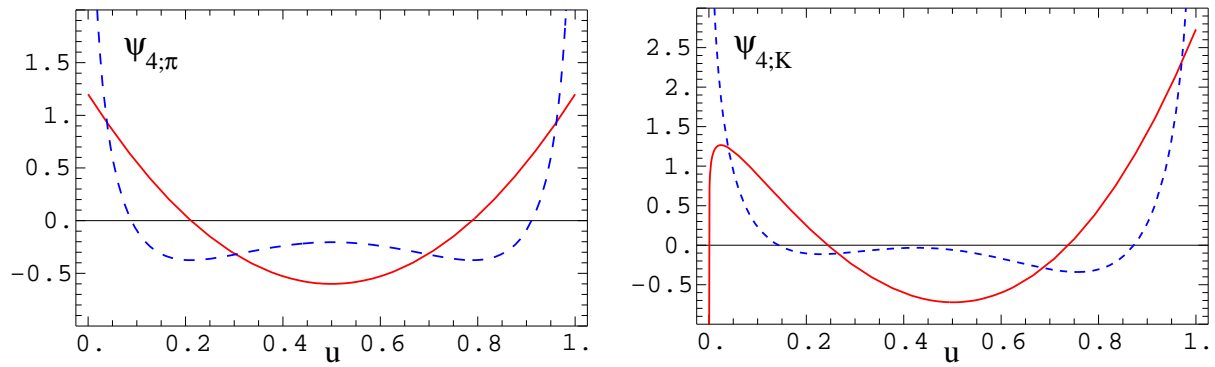
Figure 3: Same as Figure 2 for \psi_4 .
