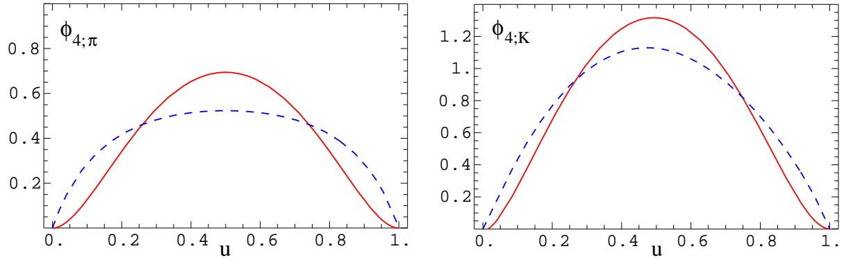
Figure 2: Left panel: \phi_{4;\pi} as a function of u for the central value of the hadronic parameters, for \mu = 1 GeV. Red (solid) line: \phi_{4;\pi} in conformal expansion, blue (dashed): \phi_{4;\pi} using the renormalon model \phi_{4;\pi}^{T4,ren} for the genuine twist-4 corrections. Right panel: same for \phi_{4;K} .
