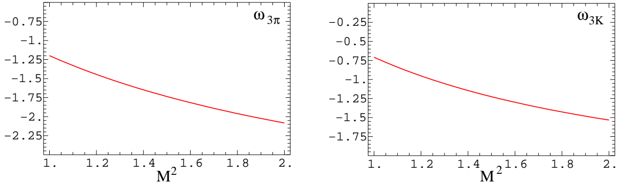
Figure 6: Left panel: \omega_{3\pi} as a function of the Borel parameter from the non-diagonal sum rule (C.13); s_0 = 0.8 \text{ GeV}^2 . Right panel: same for \omega_{3K} ; s_0 = 1.1 \text{ GeV}^2 . The results from diagonal sum rules are not shown because the gluon-condensate contribution is unknown.
