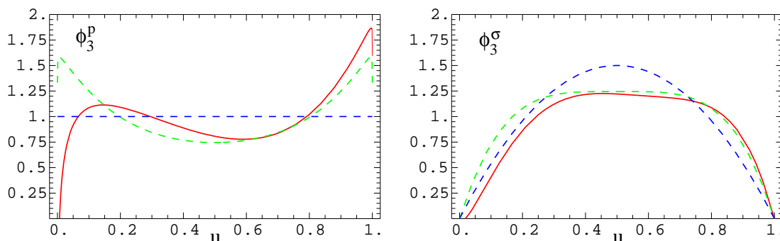
Figure 1: Left panel: \phi_3^p as a function of u for the central value of the hadronic parameters, for \mu = 1 \text{ GeV} . Red (solid) line: \phi_{3;K}^p , green (long dashed): \phi_{3;\pi}^p , blue (short dashed): asymptotic DA. Right panel: same for \phi_3^\sigma .
