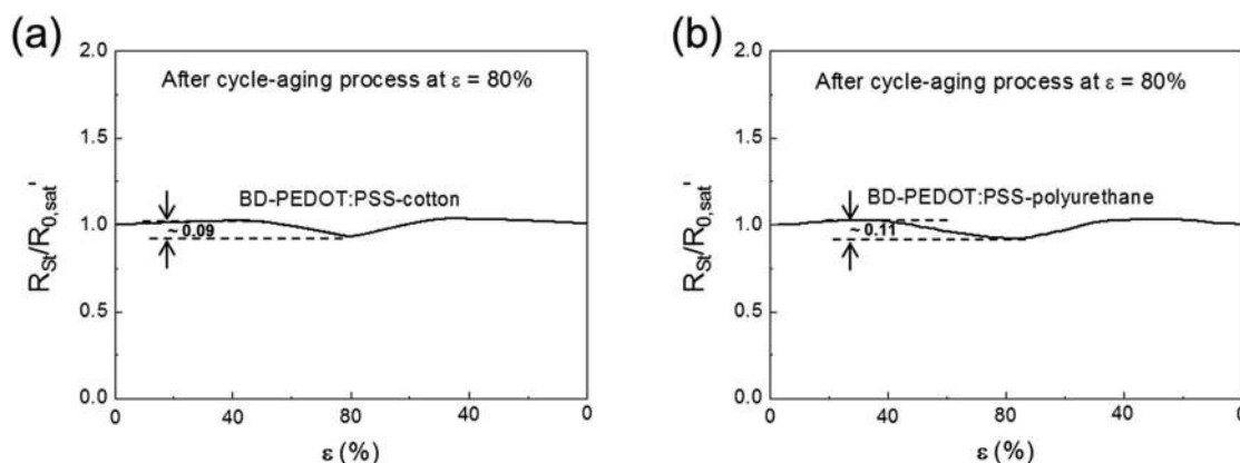
Fig. 8 The R_{Sr}/R_{0,sat}' values of (a) BD-PEDOT:PSS-cotton and (b) BD-PEDOT:PSS-polyurethane during a cycle of 80% loading after performing the cycle-aging process at \varepsilon = 80\% .
