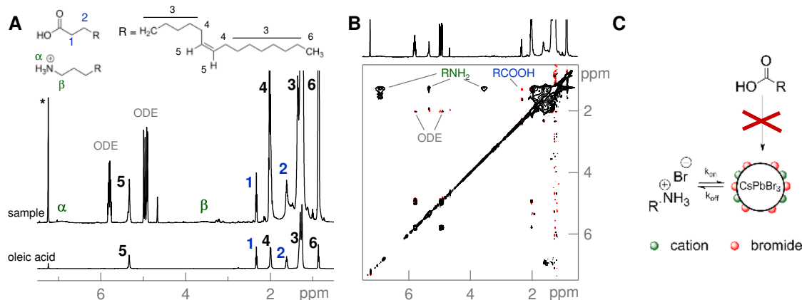
Figure 4: (A) ^1\text{H} NMR spectrum 8.4 nm \text{CsPbBr}_3 NCs purified with acetone and filtered. Concentration of QDs: 2.2\ \mu\text{M} . The reference spectrum for oleic acid is displayed and impurities of octadecene (ODE) are also indicated. (B) NOESY spectrum of the sample purified with acetone in \text{CDCl}_3 . (C) Schematic representation of the dynamic surface stabilization by oleylammonium bromide. Oleic acid is not part of the ligand shell.
