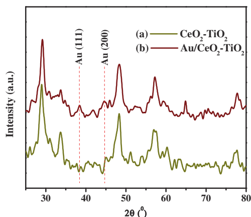
Figure 1. XRD patterns of (a) CeO 2 -TiO 2 , and (b) Au/CeO 2 -TiO 2 nano-hybrid.
