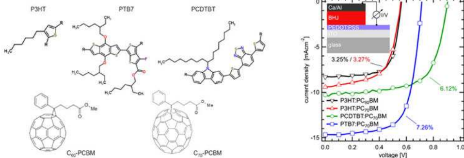
Figure 1. Left. Structures of the monomeric units of the polymers P3HT, PCDTBT, PTB7 and the fullerene derivatives C 60 -PCBM and C 70 -PCBM. Right. Current-voltage (IV) characteristics of bulk heterojunction solar cells prepared from the polymer:fullerene composites shown on the left. Numbers state the achieved power conversion efficiency (PCE). The insert schematically illustrates the device structure. Details are provided in the Supporting Information.
