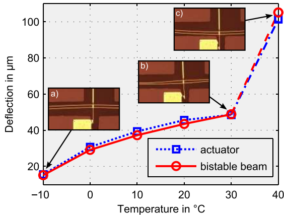
Fig. 11. The deflection of the actuator and the bistable beam, after the initial activation at -10\text{ }^{\circ}\text{C} . The device is heated up until the bistable beam switches into its second stable position at +30\text{ }^{\circ}\text{C} . The inserts depict microscope images of the bistable beam in a) its initial position, b) next to the switching point, and c) after the switching.
