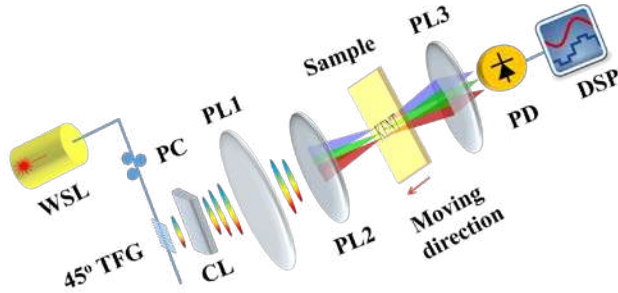
Fig. 4. Schematic diagram of the SEI system based on a 45° TFG. WSL: wavelength swept laser, PC: polarization controller, TFG: tilted fiber grating, CL: cylindrical lens, PL: plain-convex lens, PD: photo-detector, DSP: digital signal processing.
