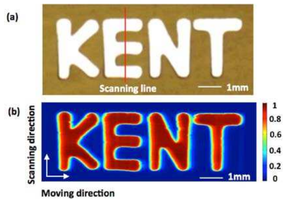
Fig. 5. (a) CCD image of the target with letters “KENT”; (b) the reconstructed dark-field 2D image obtained by the TFG-based SEI system.
