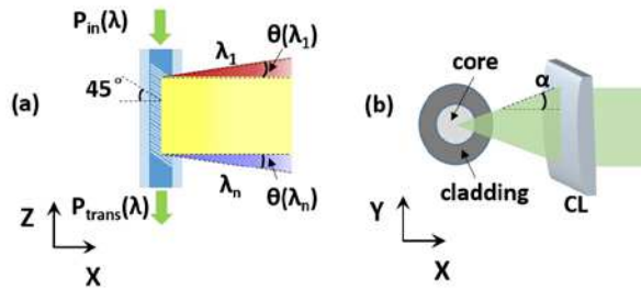
Fig. 1. Principle of a 45^\circ TFG as an in-fiber diffractive element. (a) Wavelength dependent lateral diffraction from the TFG. (b) Divergent output characteristics in radial plane. CL: cylindrical lens.
