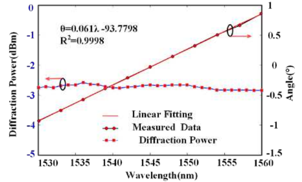
Fig. 2. Measured angular dispersion of the 45^\circ TFG (red-dotted black line) with linear fitting result (red line) and the intensity distribution of lateral diffraction (blue line).
