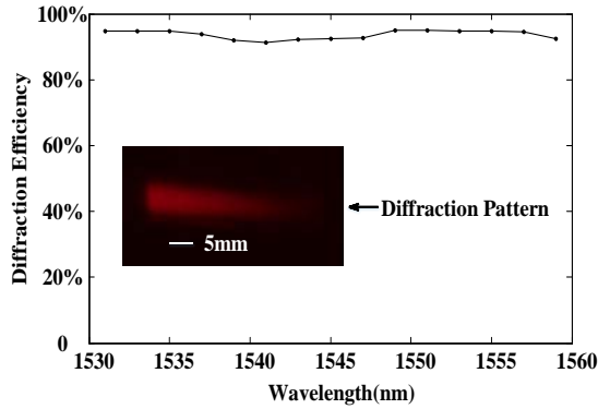
Fig. 3. Measured maximum lateral diffraction efficiency of the 45° TFG at a properly controlled polarization state. Inset: the image of diffraction pattern showing exponential decay.
