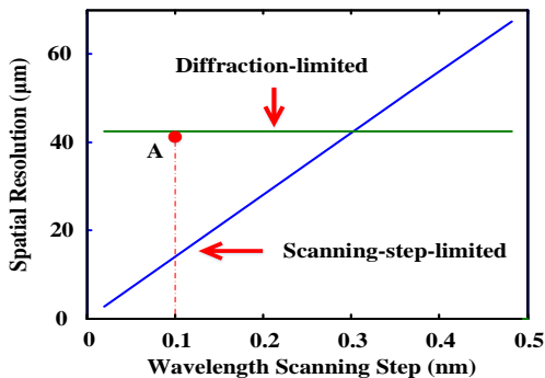
Fig. 7. Spatial resolution of our TFG-based SEI system. The diffraction-limited resolution is calculated as 43 \mu\text{m} (green line) and scanning step limited resolution is shown in blue line. Point A represents the measured system resolution of 42 \mu\text{m} .
