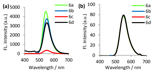
Fig. 3 Steady state emission spectra of 6a–6d (a) in solid state (spin coated: 1 wt %) (b) in chloroform ( 10^{-5} M concentration) at room temperature, \lambda_{ex} = 330 nm for fluorescence measurement.
