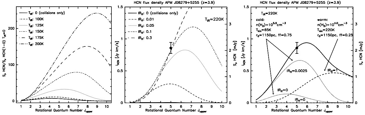
Fig. 10. Left: HCN line SED as a function of the IR radiation temperature for a \text{H}_2 density of 10^5 \text{ cm}^{-3} , a kinetic temperature of 65 K and an delution factor for the IR radiation field of 10% for each model. All SEDs are normalized to the \text{HCN}(1-0) flux density for the pure collisional excitation model ( T_{\text{IR}} = 0 \text{ K} ). The plot exemplifies the large effect of IR pumping on the HCN excitation for dust temperatures above \sim 100 \text{ K} . Middle: HCN excitation in APM08279+5255 for gas parameters as derived from the single component dust/CO model ( n(\text{H}_2) = 10^{4.2} \text{ cm}^{-3} , T_{\text{IR}} = T_{\text{kin}} = 220 \text{ K} and r_0 = 790 \text{ pc} ) as a function of the IR filling factor. For \text{IR}_{\text{ff}} = 10\% or above the IR pumping boosts the HCN excitation such that the \text{HCN}(5-4) flux density is in agreement with the observations. Right: HCN excitation model for the two-component dust/CO model for APM 08279+5255. The dashed line represents the “warm” gas with and IR illumination factor of unity, the dotted lines the “cold”, dense gas with pure collisional excitation ( \text{IR}_{\text{ff}} = 0 ) and with an IR illumination of 0.25%. The solid line the sum of both IR illuminated components. The IR radiation temperature for both components is 220 K.
