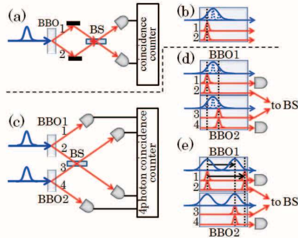
Fig. 1. (a) Schematic of Hong-Ou-Mandel interferometer between photons in a pair. (b) Since photons in a pair are generated from a single pump photon, no timing-jitter occurs. (c) Schematic of Hong-Ou-Mandel interferometer between photons in different pairs. (d) The timing-jitter caused by non-zero pulse duration. The photon pairs are generated in the front side (left side) in BBO1 and in the back side (right side) in BBO2. Thus, the input photons has the timing jitter. (e) The timing-jitter caused by GVM. Since the daughter photons propagate faster than the pump light (GVM), the timing-jitter occurs between photons in different pairs.
