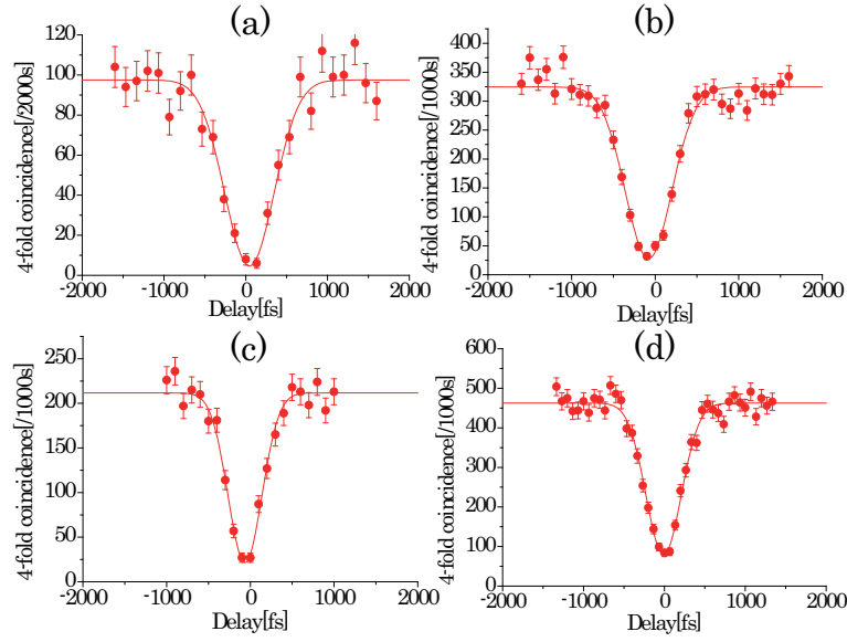
Fig. 4. HOM dips between photons in different pairs. (a) 0.7-mm BBO with 2-nm band-pass filters, (b) 0.7-mm BBO with 4-nm band-pass filters, (c) 1.5-mm BBO with 2-nm band-pass filters, and (d) 1.5-mm BBO with 4-nm band-pass filters.
