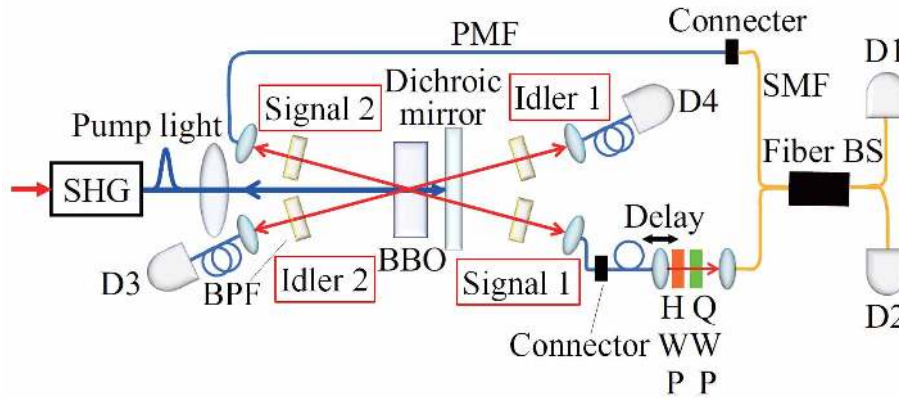
Fig. 2. Experimental setup of HOM interferometer between independent photons. SHG: second harmonic generation; PMF: polarization maintaining fiber; SMF: single-mode fiber; HWP (QWP): half (quarter) wave plate; SPCM: single-photon counting module.
