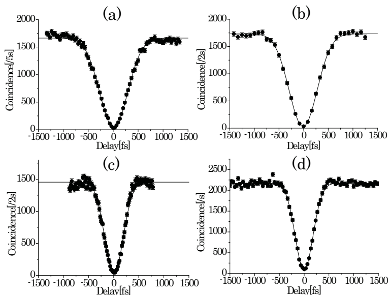
Fig. 3. HOM dips between daughter photons. The HOM dips are between Signal 1 and Idler 1 in Fig. 2 and with four different conditions (a) 0.7-mm BBO with 2-nm band-pass filters, (b) 0.7-mm BBO with 4-nm band-pass filters, (c) 1.5-mm BBO with 2-nm band-pass filters, and (d) 1.5-mm BBO with 4-nm band-pass filters.
