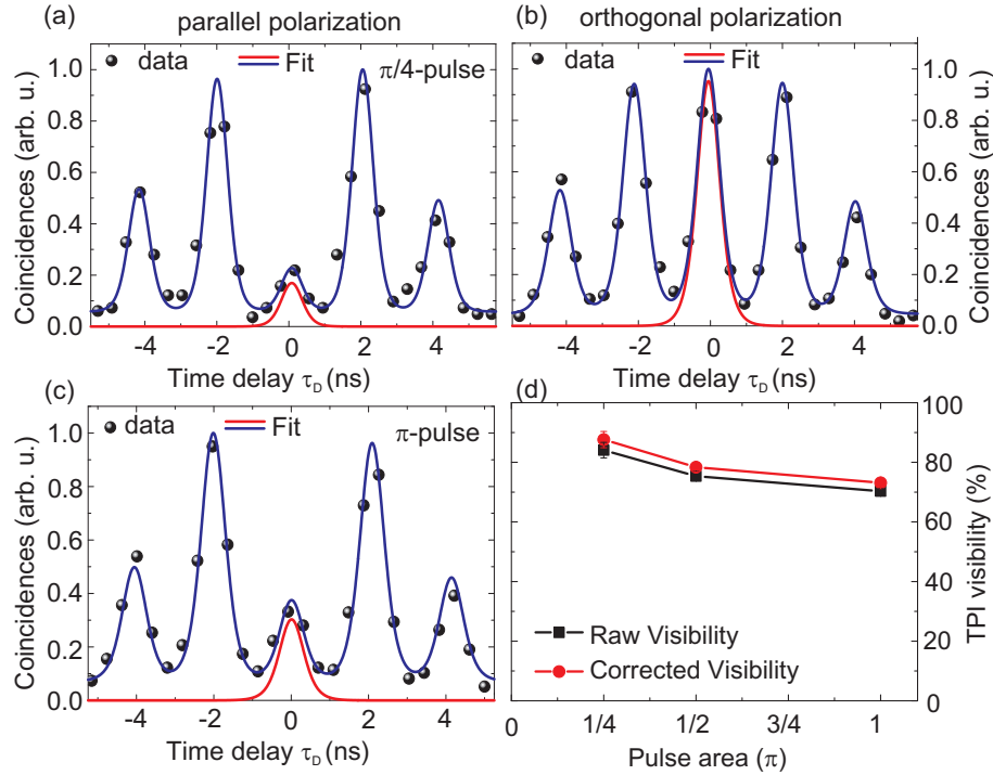
Fig. 4. Measured two-photon interference (TPI) histograms for (a) parallel polarization of both photons and driving the system with a \pi/4 -pulse and (b) orthogonal polarization. We fit each histogram with a sum of five two sided exponential functions each convolved with a Gaussian distribution and extract a visibility of v = (88 \pm 3) \% . (c) We observe a slight decrease of the TPI visibility to (73 \pm 1) \% for \pi -pulse excitation. (d) Summary of the TPI visibility versus the pulse area.
