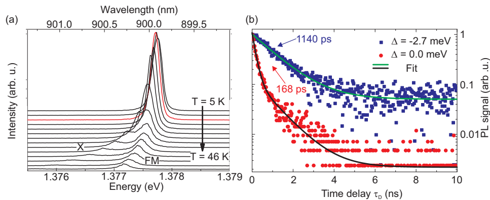
Fig. 2. (a) Temperature dependent spectras of an insitu defined micropillar with a diameter of d \approx 3 \mu\text{m} under above bandgap excitation. A strong enhancement on spectral resonance between fundamental mode (FM) and QD due to the Purcell effect is observed. (b) Time resolved measurements on and off resonance reveal a Purcell factor of F_P = 5.8 \pm 0.2 .
