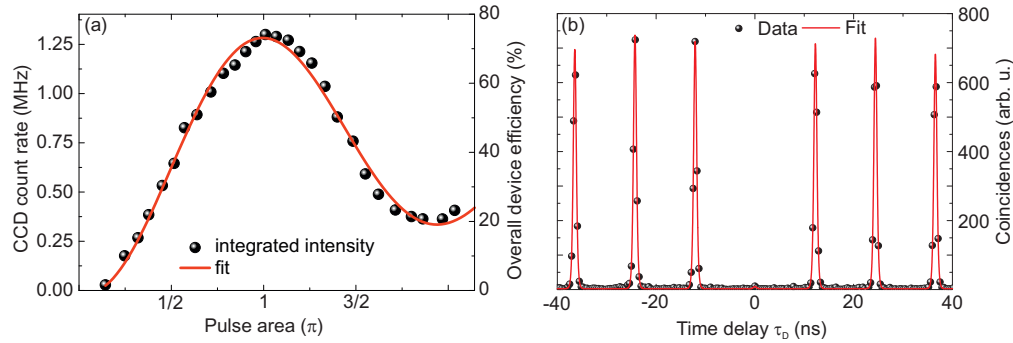
Fig. 3. (a) Measured source efficiency and count rate on the monochromator CCD versus the pulse area of the driving laser field for spectral resonance between QD and cavity mode. The fit is a damped sinusoidal function. We extract an overall device efficiency of \eta = (74 \pm 4) %. (b) 2^{nd} order auto-correlation histogram for pulsed resonant excitation with a \pi -pulse. We extract a g^{(2)} -value as low as g^{(2)}(0) = 0.0092 \pm 0.0004 .
