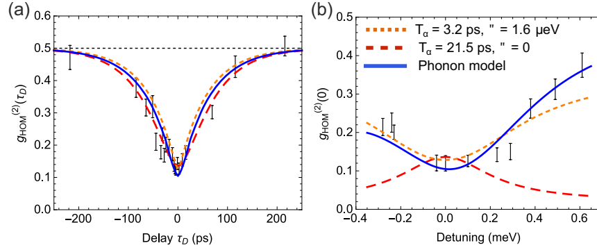
Fig. 1. (a) Two-photon-interference versus the time delay between both arms of the Mach-Zehnder-interferometer. (b) TPI-minimum versus the QD-cavity-detuning. Both curves are fitted by a microscopic model.
