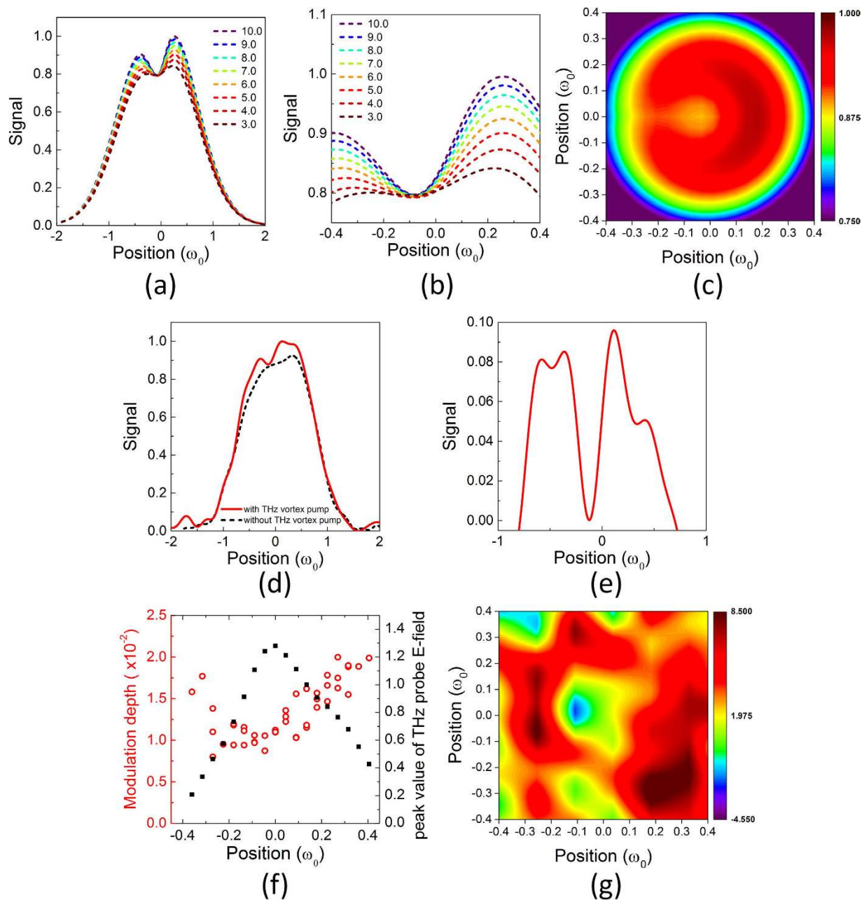
Figure 4. (a,b) Simulated spatial forms of the signal beam I_{\text{signal}}(r) at various peak intensities of the vortex pump ( 3I_s – 10I_s ). (c) Simulated 2-dimensional spatial form of the vortex pump beam at a vortex pump peak intensity of 4I_s . (d) Experimental spatial form of the signal beam with or without vortex pump beam ( \omega_0 = 8 mm). (e) The linear absorption signal defined as the intensity difference between the signal beams with and without the vortex pump. (f) Experimental modulation depth of the signal electric field with or without vortex pump beam ( \omega_0 = 11 mm). (g) Experimentally observed modulated 2-dimensional spatial form with or without vortex pump beam ( \omega_0 = 11 mm).
