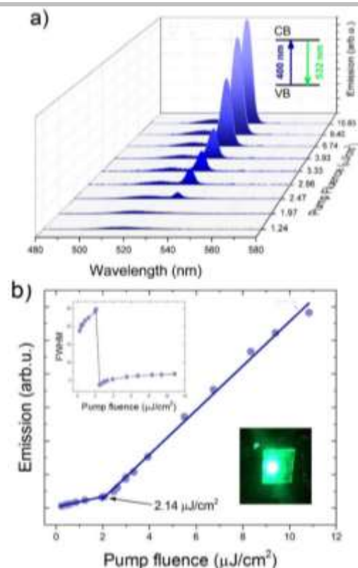
Figure 4. Pump-fluence dependent PL emission (evolution of ASE) from CsPbBr 3 NC film (a) and corresponding emission intensity at 530 nm (b), and FWHM (inset of b). All the spectra are obtained with 400 nm femtosecond laser excitation.
