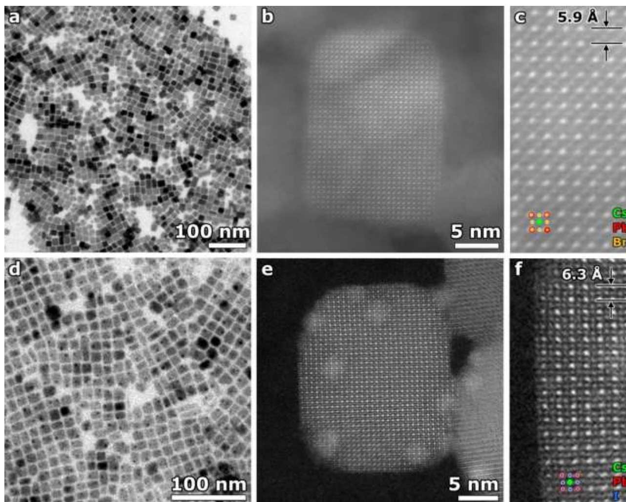
Figure 2 (a,d) BF-TEM overview images of CsPbBr 3 and CsPbI 3 NCs, respectively. (b,e) Atomically resolved high resolution HAADF-STEM image of a single CsPbBr 3 and a CsPbI 3 NC with (c,f) a more detailed view, respectively.
