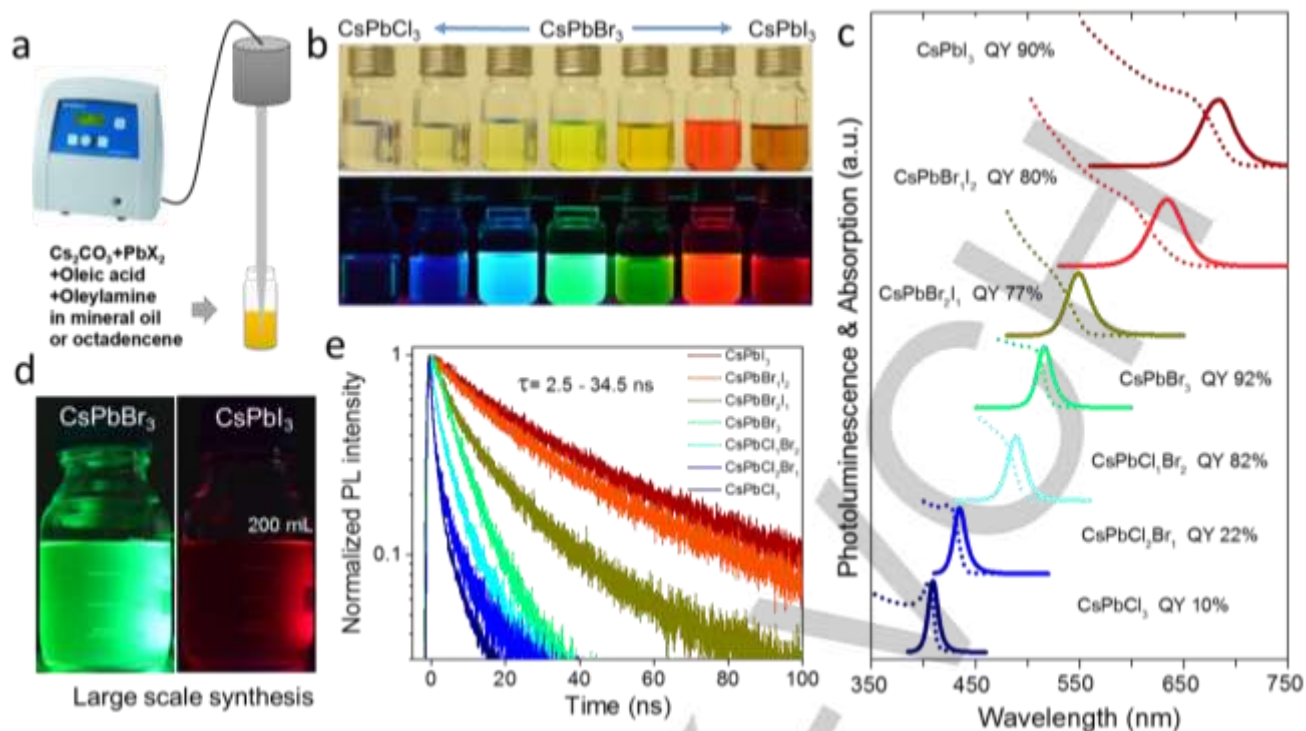
Figure 1. (a) Schematic illustration of the synthesis of \text{CsPbX}_3 NCs through single-step tip-sonication. (b) Photograph of colloidal dispersions of \text{CsPbX}_3 NCs with different halide ( x = \text{Cl}, \text{Br} and \text{I} ) compositions in hexane under room light (top) and UV light (bottom, \lambda = 367 nm). (c) Corresponding UV-vis and PL spectra, and PLQYs of samples shown in (b). (d) Scalable synthesis of NCs (scaled up to 10 times). Photograph of \text{CsPbBr}_3 and \text{CsPbI}_3 colloidal dispersions under UV light. (e) PL decay dynamics of NCs shown in (b) (calculated \tau \sim 2.5 -34.5 ns).
