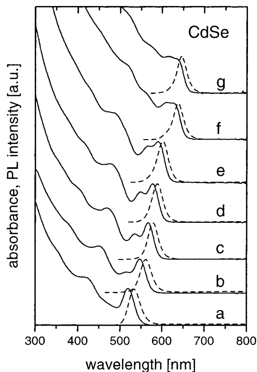
Figure 1. Room-temperature absorption and emission spectra of CdSe nanocrystals monitored during the growth at 300 °C.
