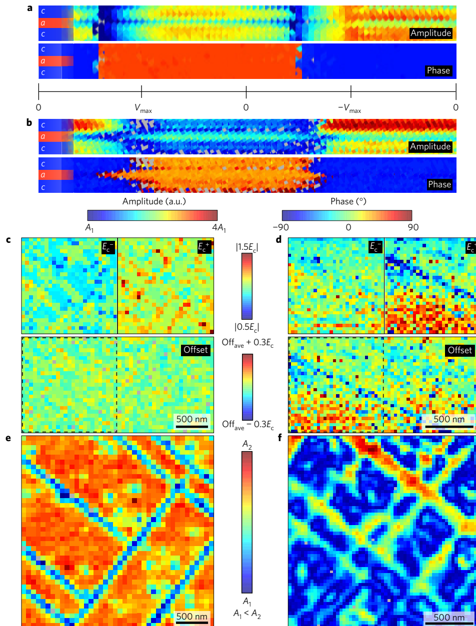
Figure 5 | Breaking down the differences between homogeneous and compositionally graded heterostructures. a, b , Voltage-lapse images near an a domain in homogeneous \text{PbZr}_{0.2}\text{Ti}_{0.8}\text{O}_3 ( a ) and compositionally graded \text{PbZr}_{1-x}\text{Ti}_x\text{O}_3 ( b ) heterostructures as imaged throughout a switching cycle. c, d , Negative coercive field ( E_c^- ), positive coercive field ( E_c^+ ) and voltage offset for the same homogeneous \text{PbZr}_{0.2}\text{Ti}_{0.8}\text{O}_3 ( c ) and compositionally graded \text{PbZr}_{1-x}\text{Ti}_x\text{O}_3 ( d ) heterostructures extracted from fits of piezoelectric hysteresis loops. Colour scales based on an identical fraction of the average fitted coercive field. e, f , High-field, local piezoresponse of the same homogeneous \text{PbZr}_{0.2}\text{Ti}_{0.8}\text{O}_3 ( e ) and compositionally graded \text{PbZr}_{1-x}\text{Ti}_x\text{O}_3 ( f ) heterostructures revealing inverted responses between the two heterostructure variants. All scale bars are 500 nm.
