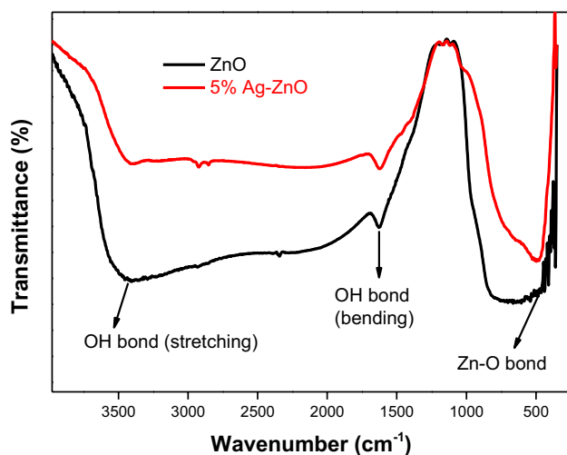
Fig. 6 FTIR spectra of ZnO and Ag-ZnO NPs synthesized by Azadirachta indica gum
