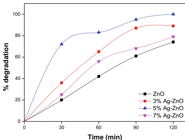
Fig. 10 Photocatalytic degradation of methylene blue with different catalysts
