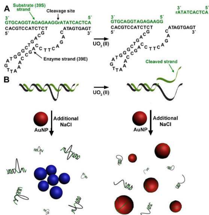
Figure 5. (A) The design and sequence of the label free sensor (complex). After \text{UO}_2^{2+} induced cleavage, 10 mer ssDNA is released which adsorbs on AuNP surface. (B) AuNP reaction in addition of \text{UO}_2^{2+} treated/untreated complex and additional NaCl. AuNPs aggregate in the absence of \text{UO}_2^{2+} but remain dispersed in its presence.
