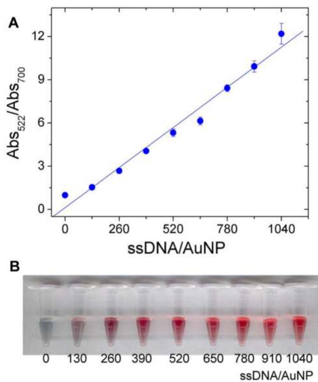
Figure 6. (A) Extinction ratio dependence on the number of 10 mer ssDNA per 13 nm AuNP. The stability of AuNP increases as more ssDNA exist per one AuNP. (B) The color change of AuNPs with different ratio of DNA per AuNP.
