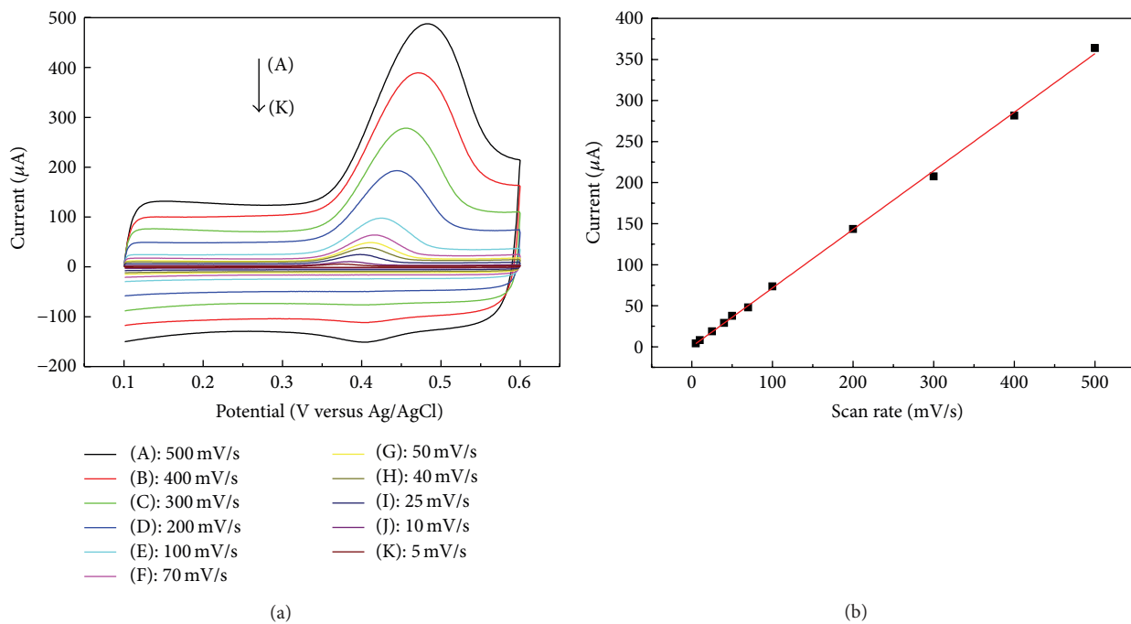
FIGURE 6: (a) Cyclic voltammograms in 0.1 M PBS (pH 7.4) containing 5 μM 8-OHdG at different scan rates from 5 mV/s to 500 mV/s on the SWCNTs-Nafion/GCE. (b) Dependence of the peak current on the scan rates from 5 mV/s to 500 mV/s.
