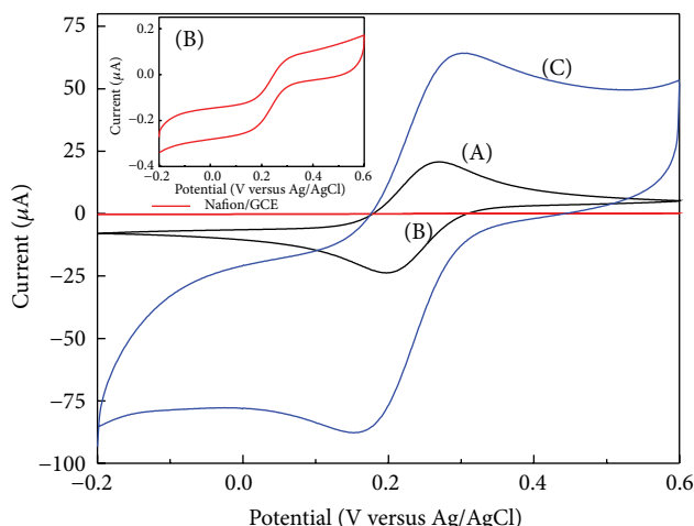
FIGURE 4: Cyclic voltammograms on different electrodes at a scan rate of 50 mV/s in 0.1 M PBS (pH 7.4) containing 5.0 mM \text{K}_3\text{Fe}(\text{CN})_6 –5.0 mM \text{K}_4[\text{Fe}(\text{CN})_6] . (A) Bare GCE, (B) Nafion/GCE, and (C) SWCNTs-Nafion/GCE.
