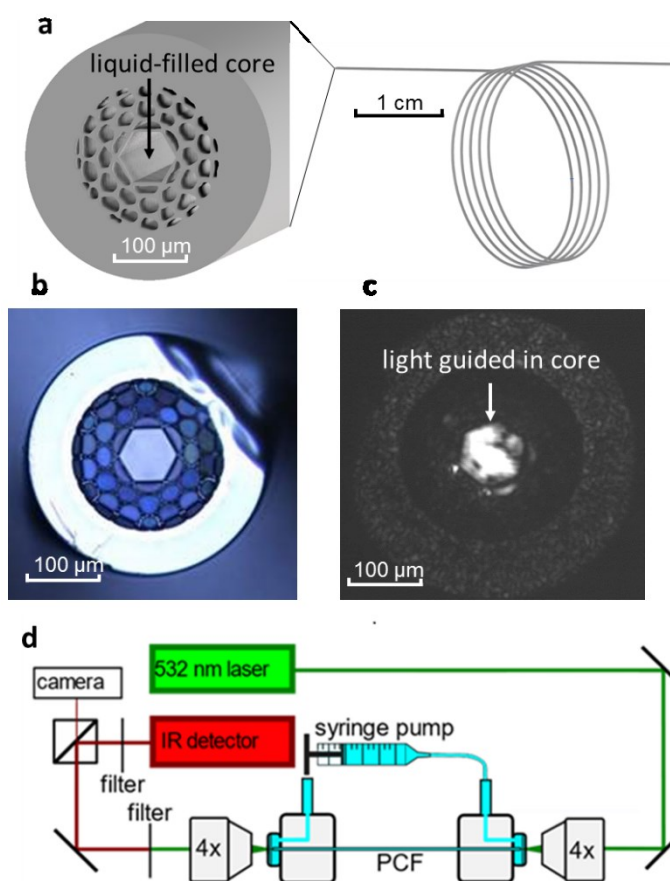
Figure 1. (a) Schematic illustration of a hollow-core photonic crystal fibre. (b) Image of the end-face of the large-core HC-PCF used in this study; this is a kagomé-type HC-PCF, named after the particular lattice arrangement in the cladding structure. (c) Image of the end face of the HC-PCF, showing confinement of the 532-nm laser beam to the core region. (d) Schematic diagram of the experimental system.
