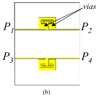
FIGURE 1. Sketch showing the working principle of the proposed sensor (a) and top view of the microwave part (i.e., the pair of OCSRR-loaded lines) (b). The metal surrounding the OCSRR is short-circuited to the ground plane through vias.
