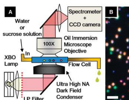
Figure 2. (A) Experimental wet environment dark-field setup designed for single nanoparticle spectroscopy in various surrounding media. (B) Typical dark-field image of the nanoparticles; the scale bar is 10 \mu\text{m} .
