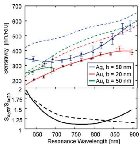
Figure 3. (Top) Experimental results (continuous lines) and BEM-simulation without substrate (dashed lines) of single-particle sensitivity of silver (blue line), 20 nm thick (red line), and 50 nm thick (green line) nanorods. The error bars indicate the uncertainty of the mean in a range of 25 nm. (Bottom) The experimentally obtained (continuous line) and BEM-simulated (dashed line) sensitivity enhancement ( S_{Ag50}/S_{Au20} ) of silver nanorods with 50 nm thickness in relation to gold nanorods with 20 nm thickness.
