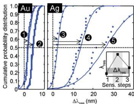
Figure 4. Cumulative distribution of single nanoparticle resonance wavelength shifts after one sensing measurement cycle (the sensing cycle shift). The continuous lines are Gaussian fits, the arrow indicates the mean cycle shift. Left graph: (1) small Au rods with 610 nm long pass (LP) filter (2) small Au rods without LP filter. Right graph: (3) Ag rods with 610 nm LP filter, (4) Ag rods with 530 nm LP filter, (5) Ag rods without LP filter. Inset at bottom right: definition of sensing cycle shift \Delta\lambda_{\text{res}} in the cycle n_1 \rightarrow n_2 \rightarrow n_1 .
