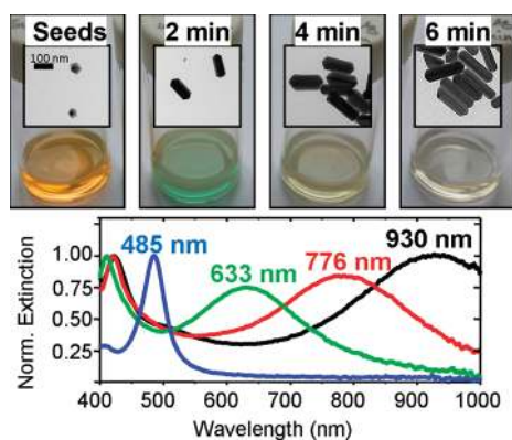
Figure 1. Representative silver nanorod samples are shown as photographs and TEM images together with the corresponding ensemble extinction spectra (bottom). The samples correspond to Ag-seeds and Ag-nanorods grown with 2, 4, and 6 min of heating time (from left to right). Their plasmon peak increases from 485 to 633, 776, and 930 nm.
