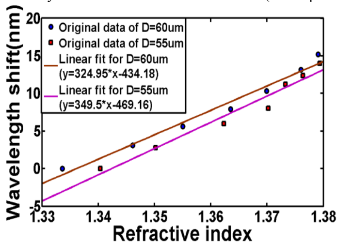
Figure 7. RI sensitivity characterization for both sensors (D=60 μm and D=55 μm)
