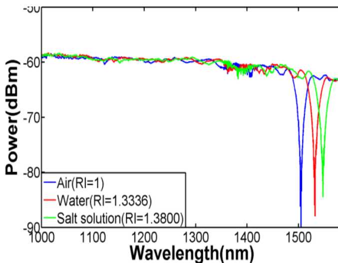
Figure 7. RI sensitivity characterization for both sensors (D=60 μm and D=55 μm)
