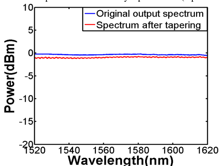
Figure 2. Transmission spectra of adiabatically tapered fiber (taper diameter: 60 \mu\text{m} )
