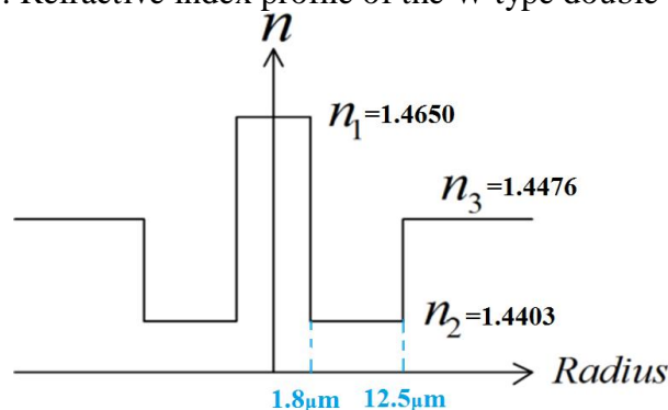
Figure 4. Refractive index profile of the W type double-clad fiber
