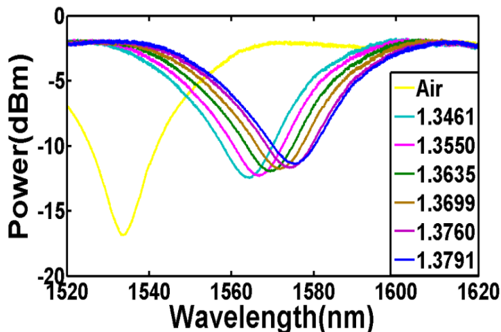
Figure 6. A broader spectrum for different external refractive index (D=55 μm)
