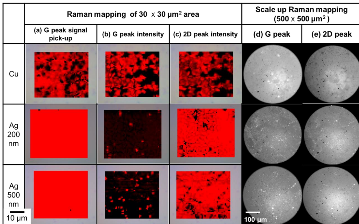
Figure S1 Spectroscopic Raman mapping of graphene characterization. (a) Signal pick-up of the G and intensity maps of the (b) G and (c) 2D band for Cu, Ag200Cu and Ag500Cu respectively with 30 x 30 \mu\text{m}^2 map area. (d-e) Scale up mapping of Raman spectroscopy with 500 x 500 \mu\text{m}^2 map area. Intensity maps of the (d) G band and (e) 2D band for Cu, Ag200Cu and Ag500Cu, respectively.
