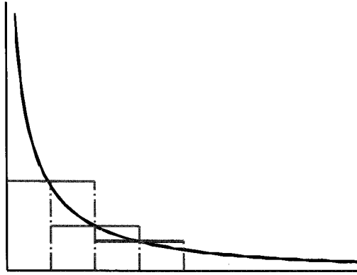
Figure 1. Riemann sums for x^{-a}/(1+x) .
