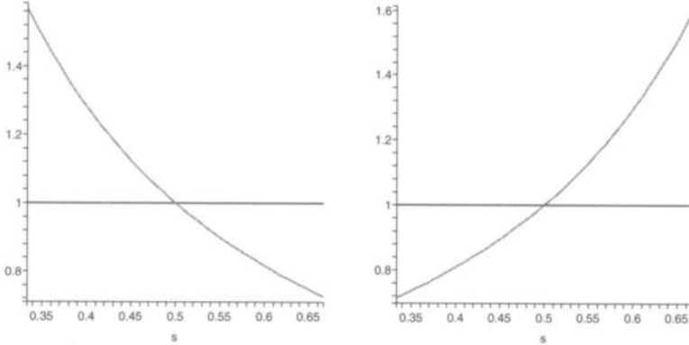
Figure 2. \mathcal{R} (left) and \mathcal{I} (right) on [1/3, 2/3] .
