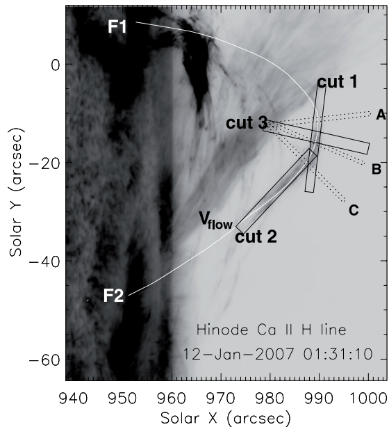
Fig. 1. Chromospheric material at 10 000–20 000 K in coronal loops observed by Hinode SOT with Ca II H emission line filter ( 3968.5 \pm 3 \text{ \AA} ). The material flows along the loops, which exhibit periodic oscillations (the movie of this event is available online). The oscillating loop studied is outlined with a white curve, which is obtained by tracing flows observed at 01:28:15, 01:31:10, and 01:34:40. The plasmas were ejected from the region F1 and moved along the loop to the other foot F2. Cuts 1 and 2 are used to measure the flow speeds (see Fig. 2), cut 3 is used to measure the transverse oscillations of the loop (see Fig. 3), and cuts A–C (dotted narrow boxes) are used to detect the wave propagation (see Fig. 4). This image and subsequent images are “negative” images, and the darkest features correspond to brightest features in SOT.
