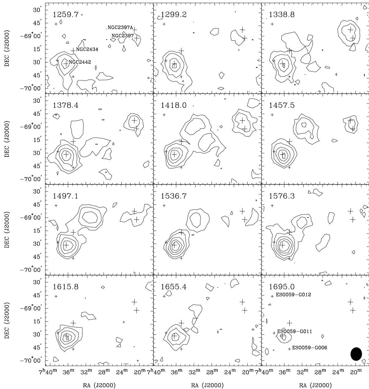
FIG. 4.—Channel maps of H I emission from the HIPASS observations of the region around NGC 2442. The contours correspond to flux densities of 15, 30, 60, 90, and 120 mJy beam -1 . For reference, the optical positions of the four major NGC galaxies in the field are marked in each panel with a large cross and identified in the first panel; three more ESO galaxies are marked with small crosses and identified in the last panel. HIPASS beam size is also indicated in the last panel.
