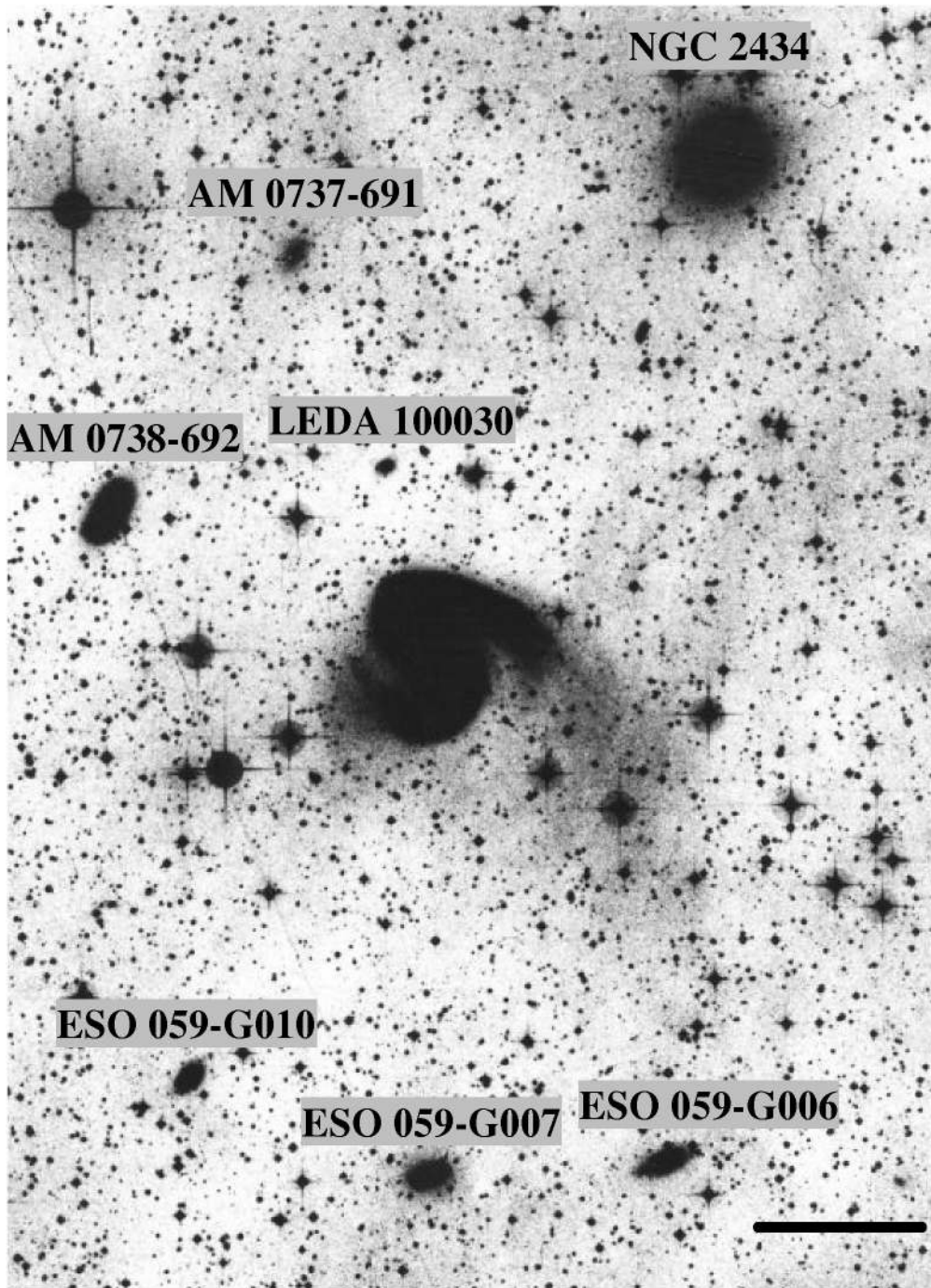
FIG. 2.—Deep optical image of the field immediately surrounding NGC 2442, obtained by summing three blue photographic plates from the UK Schmidt Telescope in the manner outlined by Malin (1981). Comparison with the surface photometry of Sérsic & Donzelli (1993) indicates that the faintest structures visible have a surface brightness of B \sim 28 mag arcsec ^{-2} . With the exception of NGC 2442 at the center, all galaxies listed in Table 1 that are visible in this image are identified by a label immediately above each one. The solid bar at lower right is 5' in length.
