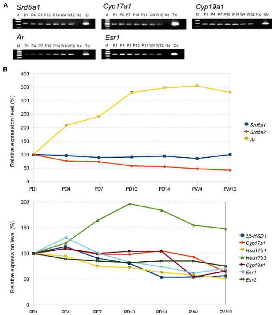
FIGURE 6 | (A) Typical electrophoresis gel images for the RT-PCR analysis for the mRNAs of sex-steroidogenic enzymes ( Srd5a1 : 5 \alpha -reductase type 1, Cyp17a1 : P450 (17 \alpha ), and Cyp19a1 : P450arom) and sex hormone receptors ( Ar : AR and Esr1 : ER \alpha ). Each band of PCR product is stained with EtBr and visualized. Lanes labeled with P1 (PD1), P4, P7, P10, P14, W4 (PW4), and W12 represent the PCR products derived from the male rat hippocampus at the corresponding ages. The left-most lane (labeled with
